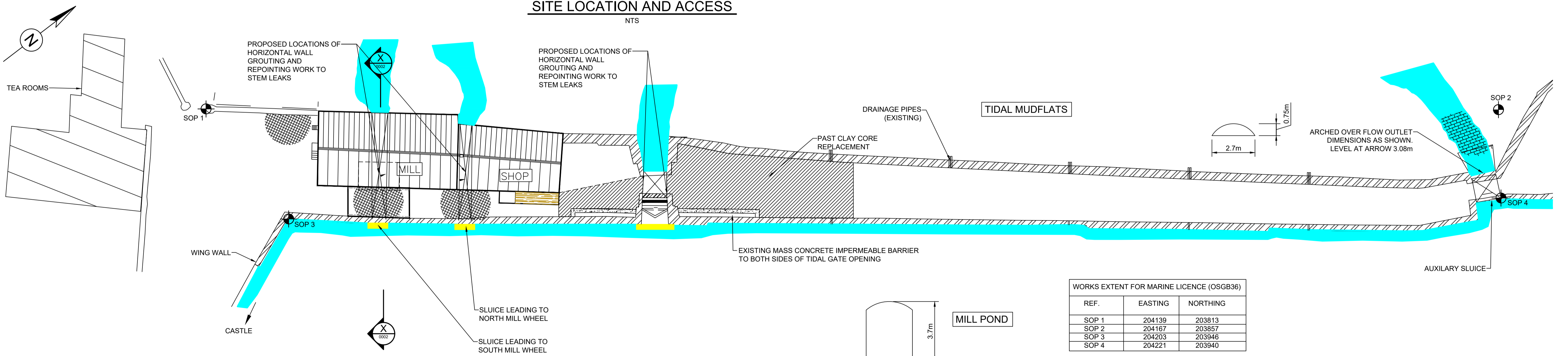
PLAN OF CAUSEWAY SHOWING REPAIR ITEMS 1:250
