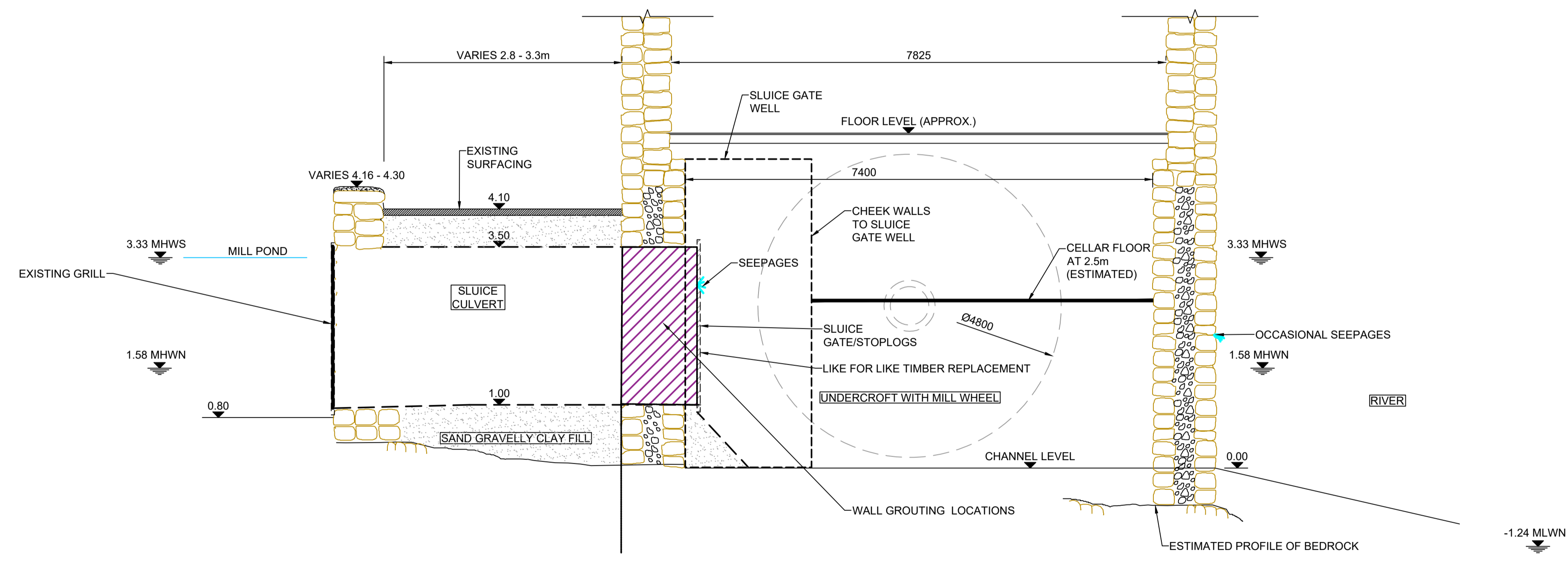
TYPICAL DETAIL OF CAUSEWAY STRENGTHENING X-X
