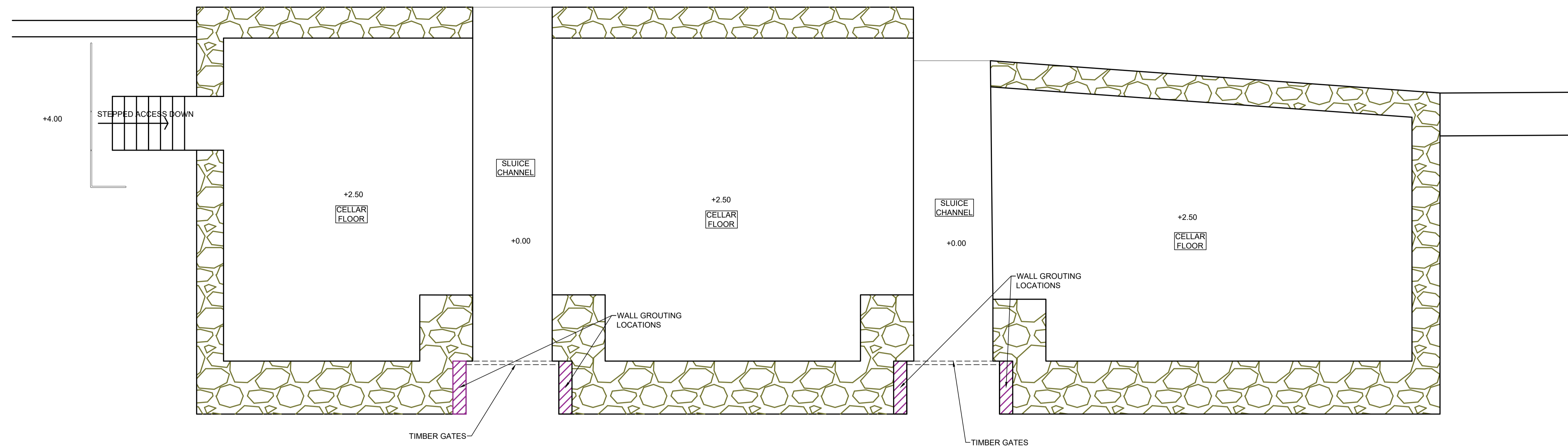
GROUTING LOCATIONS PLAN
