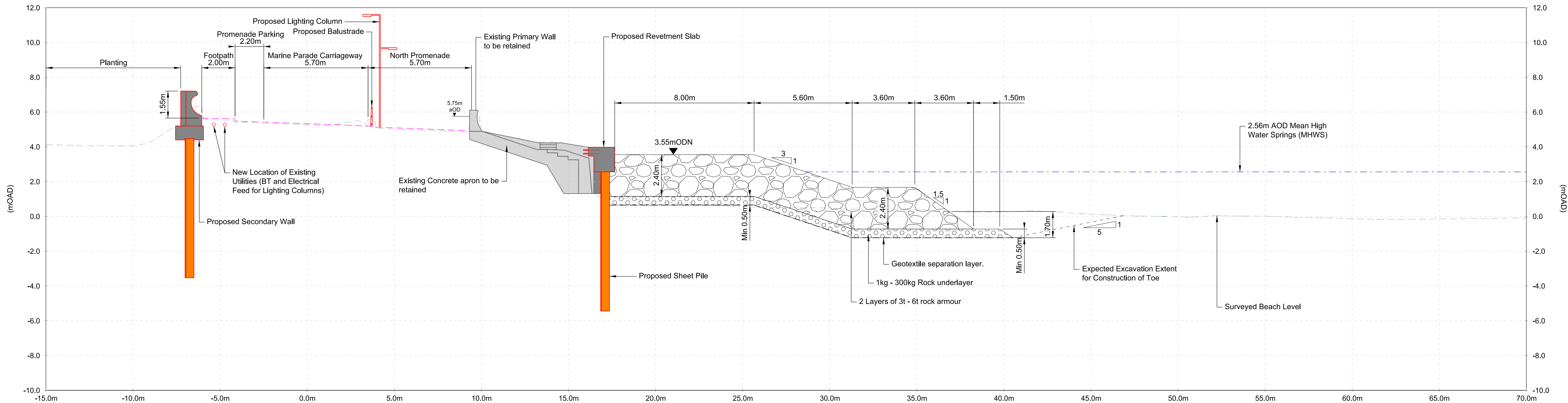
Section F-F
