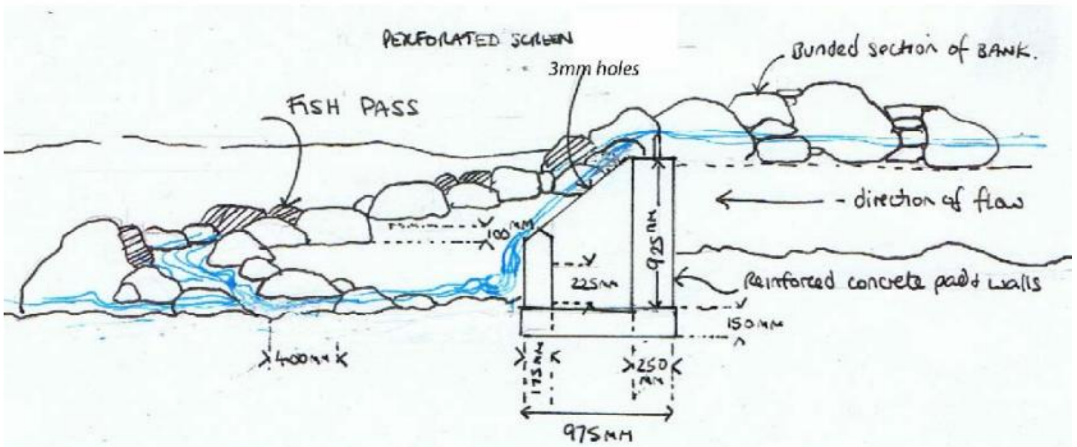
DRAWING 3b. CROSS SECTION OF INTAKE + FISH PASS.
