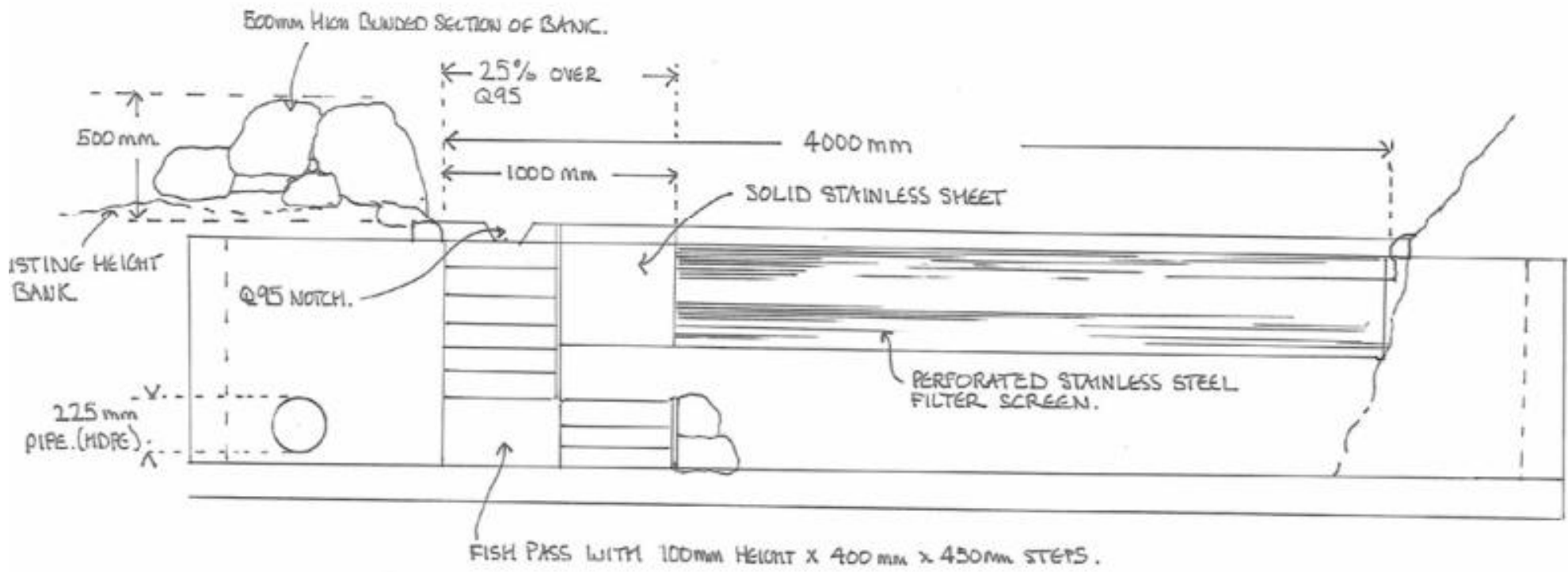
DRAWING 3a. ELEVATION OF INTAKE (AS SEEN LOOKING UPSTREAM)
