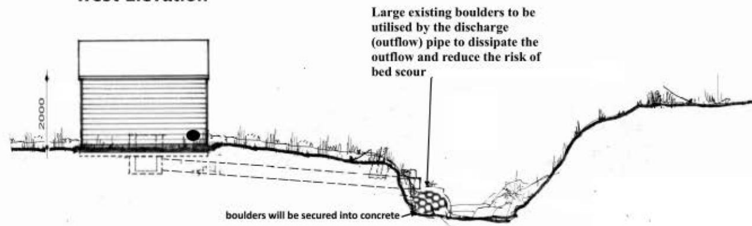
West Elevation
