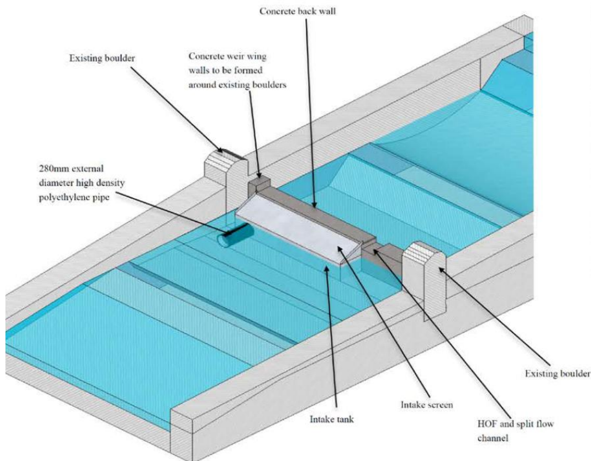
Intake - Proposed Isometric view
