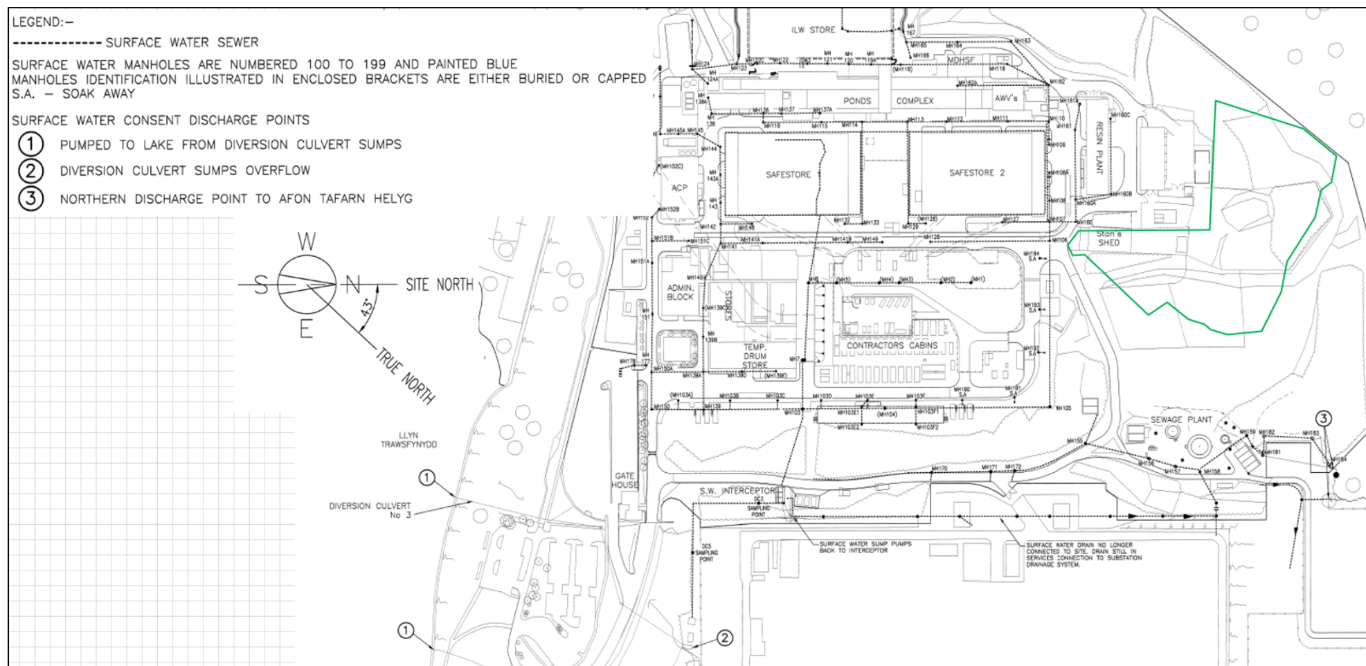
Figure 17 – Site layout plan showing DfR area (green polygon) in relation to the site surface water drainage system
