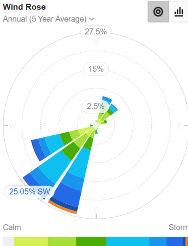
Figure 29 – Windrose from Capel Curig Weather Station (2020-2024)
