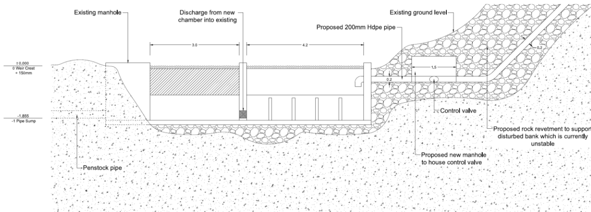
S-03 Weir Cross Section 1:50
