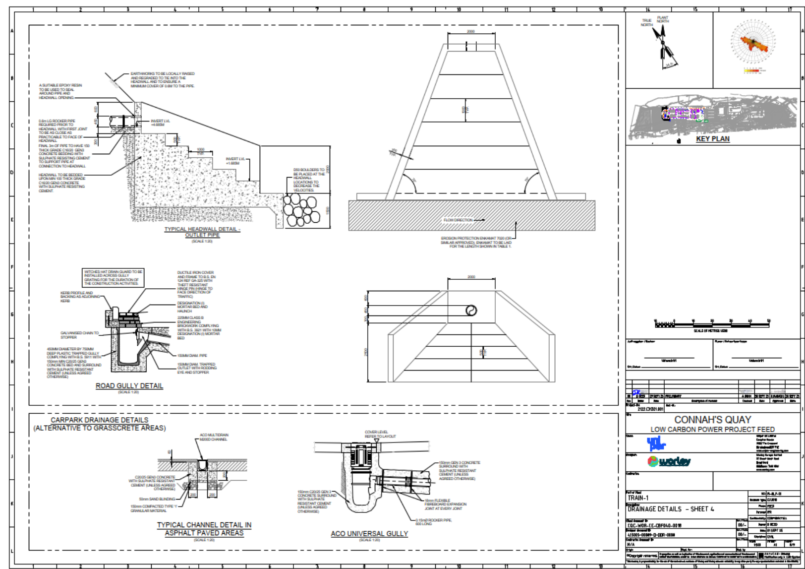
Figure 11: Indicative design of Proposed Surface Water Outfall (CQC-WOR-CE-CBF040-0018)
