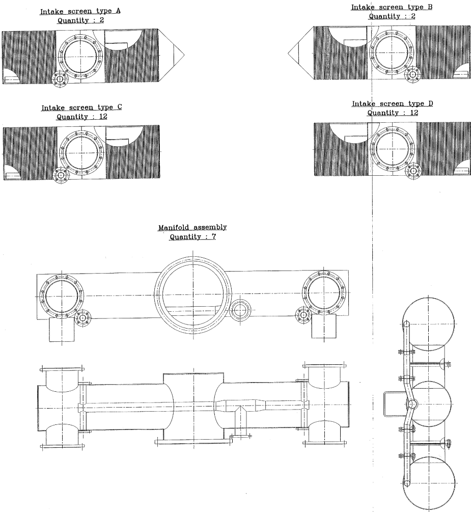
Figure 8: INTAKE SCREEN AND MANIFOLD ASSEMBLY_CNC-103556
