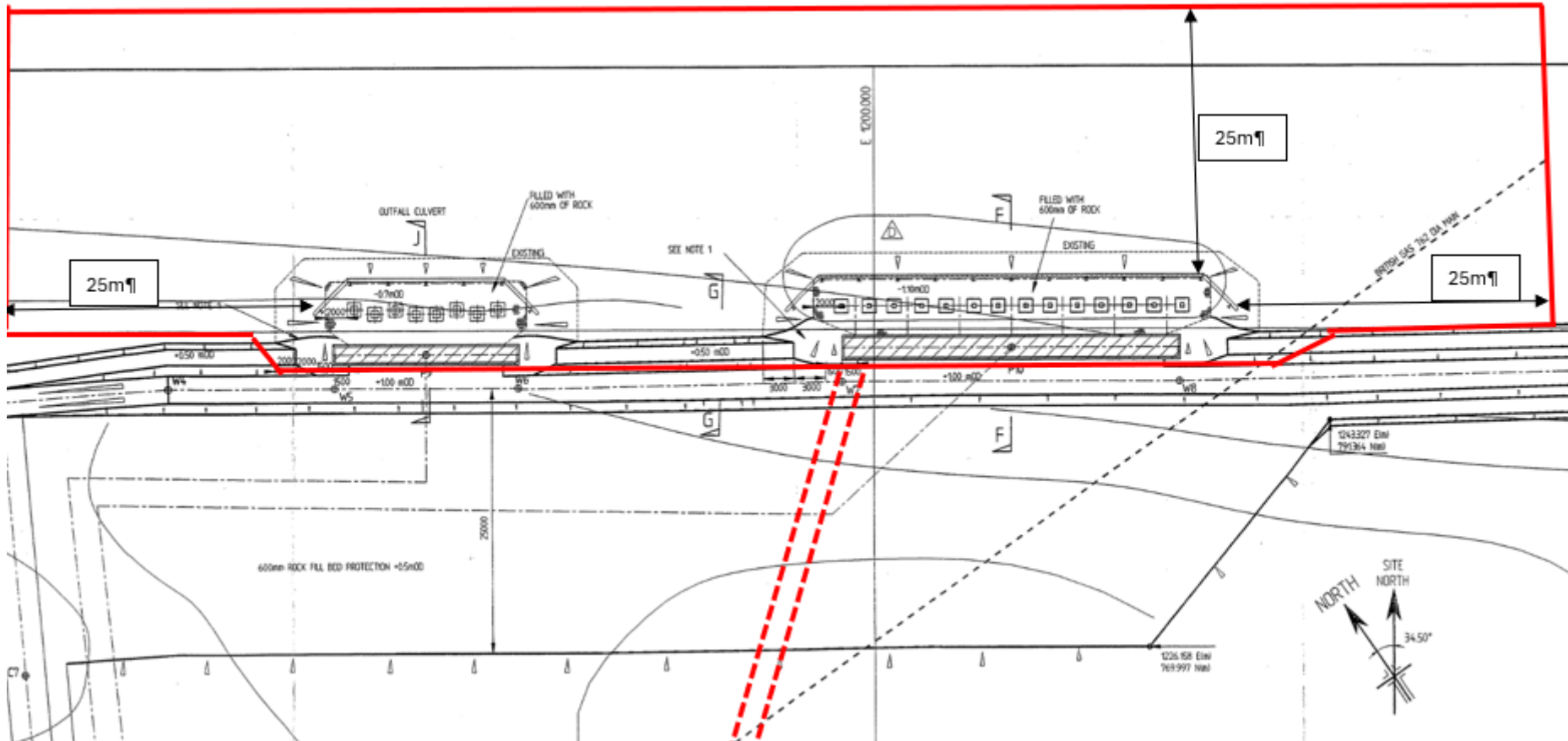
Figure 6: Indicative boat and/ or barge mooring area (annotated version of Drawing no. CNC/1M0L/GA/0/R1000/00/022)
