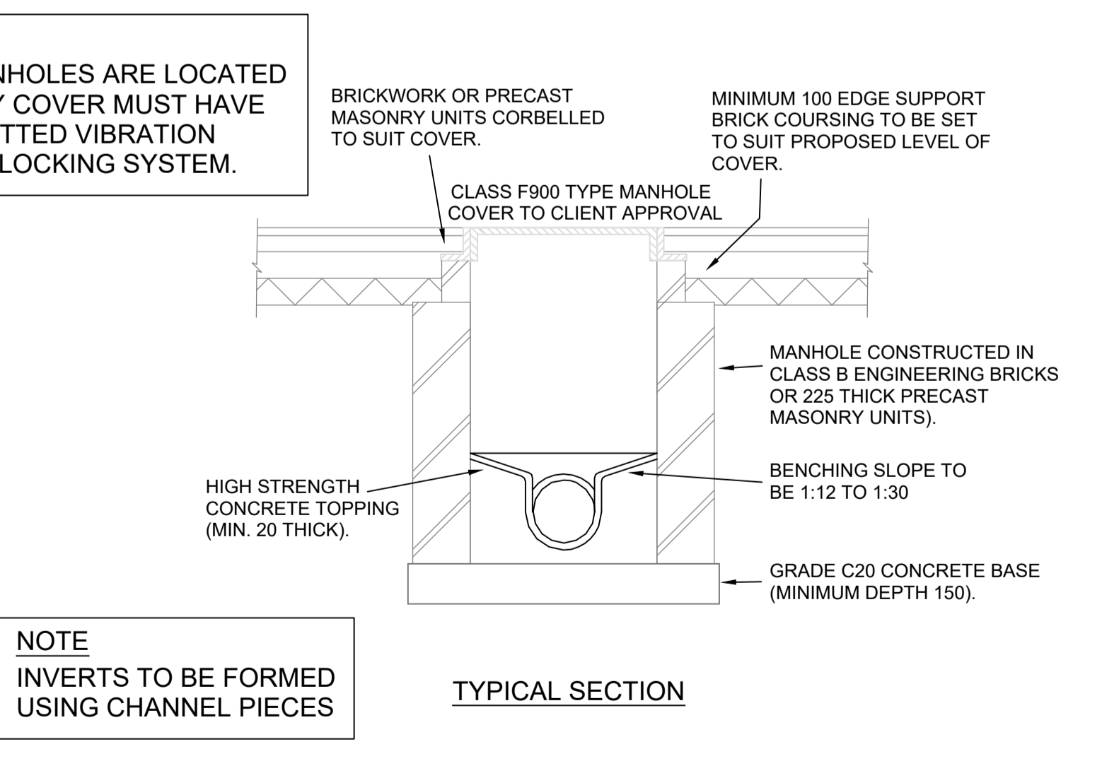
TYPICAL MANHOLE DETAILS WHERE GROUND LEVEL TO PIPE SOFFIT LESS THAN 1.5m
