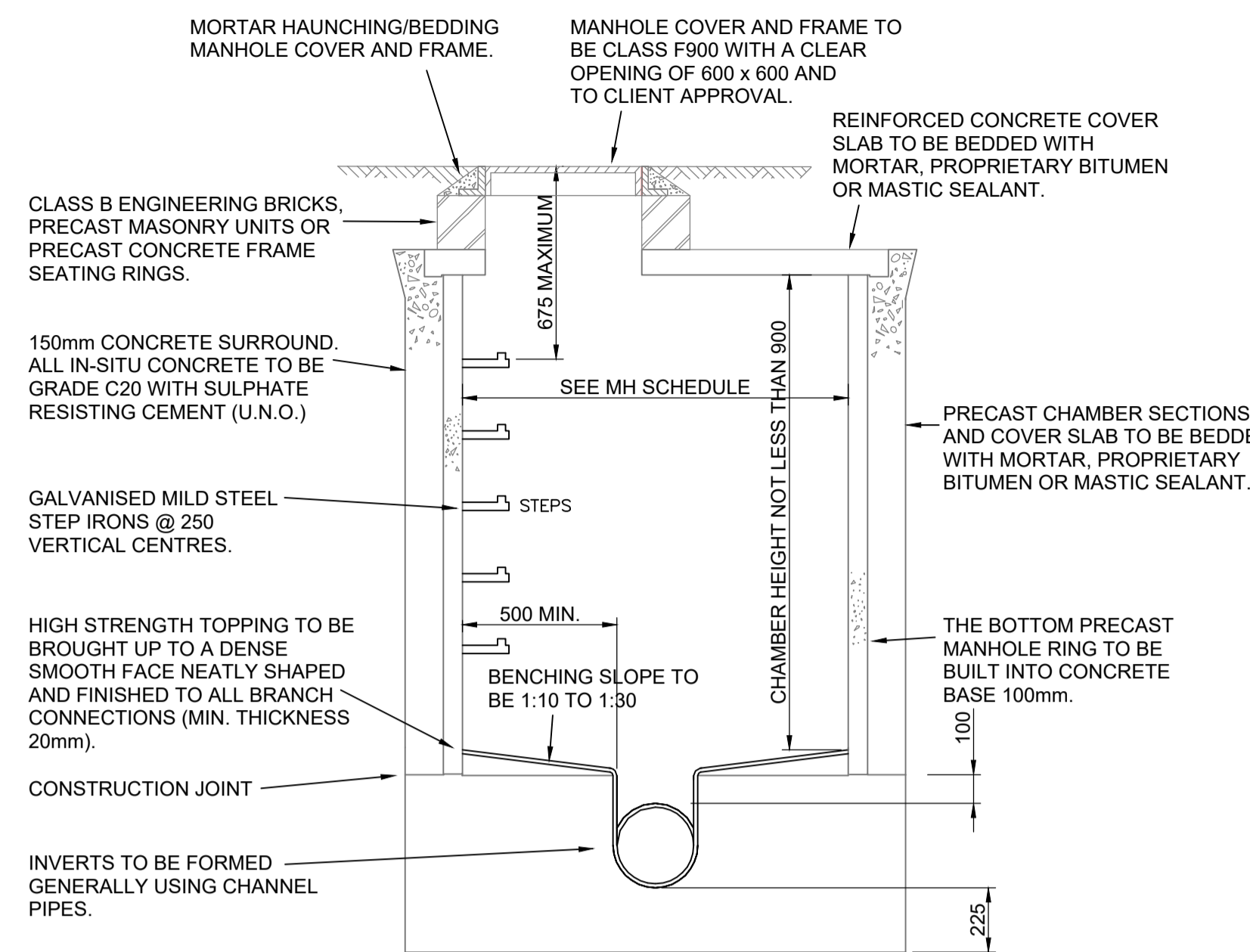
TYPICAL MANHOLE DETAILS (GROUND LEVEL TO SOFFIT OF PIPE < 3m)
