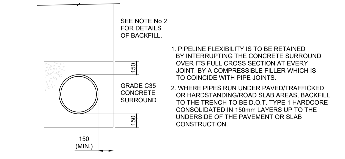
TYPICAL PIPE BEDDING DETAIL WHERE COVER FROM GROUND TO PIPE SOFFIT LESS THAN 1200mm
