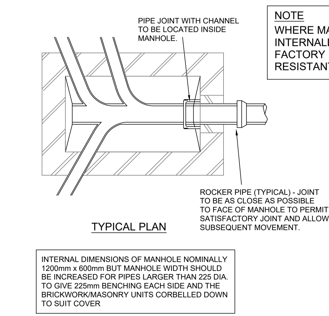
TYPICAL MANHOLE DETAILS WHERE GROUND LEVEL TO PIPE SOFFIT LESS THAN 1.5m
