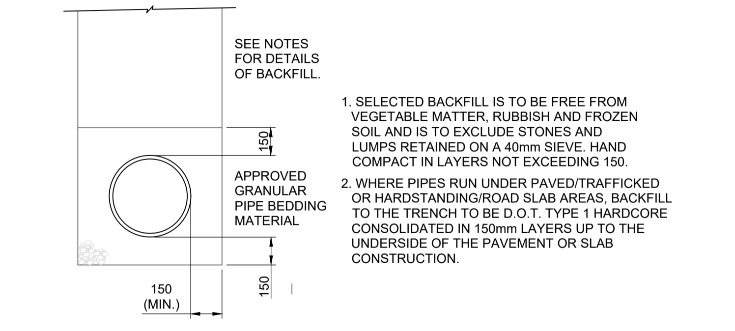
TYPICAL PIPE BEDDING DETAIL WHERE COVER FROM GROUND TO PIPE SOFFIT GREATER THAN 1200mm
