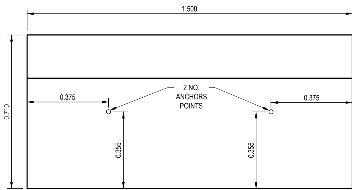
COPING STONE - REINFORCED CONCRETE WALL - PLAN SCALE 1:10
