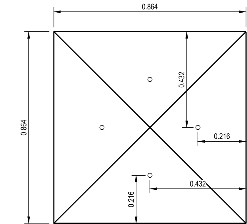
COPING STONE - FLOOD GATE COLUMN - PLAN SCALE 1:10
