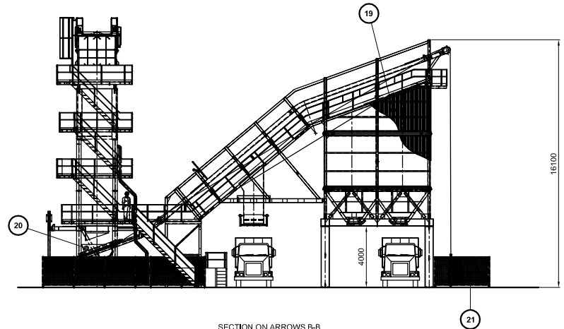
SECTION ON ARROWS B-B
