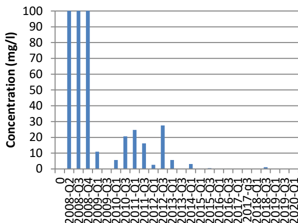
TMS monitoring - Timber Pond
