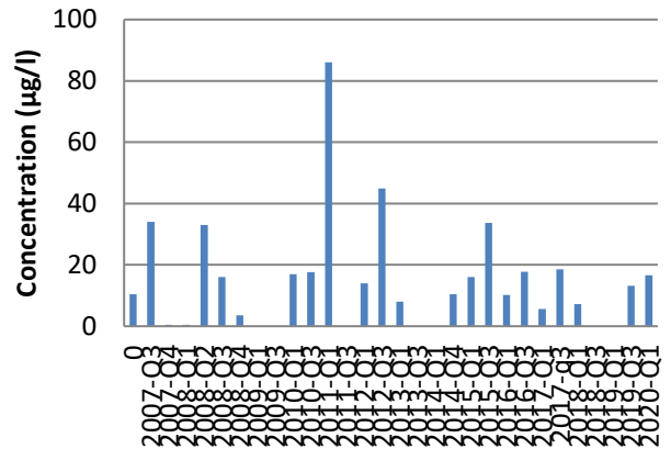
Copper monitoring - SW3
