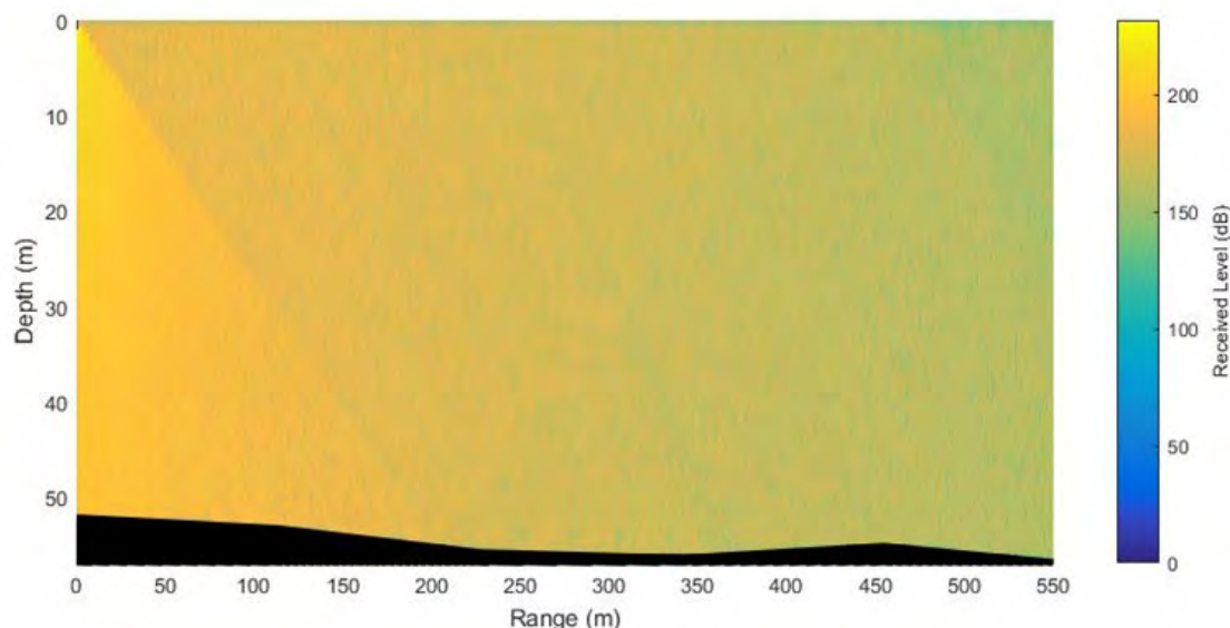
Figure 3-4 BH results during summer months for a multi-beam echosounder; received sound field for a depth/range slice at location 1. Bathymetry is shown in black.
