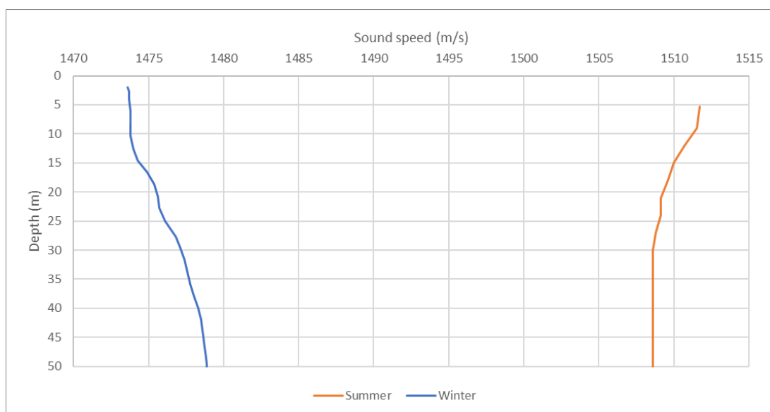
Figure 3-2 Summer and Winter sound speed profiles
