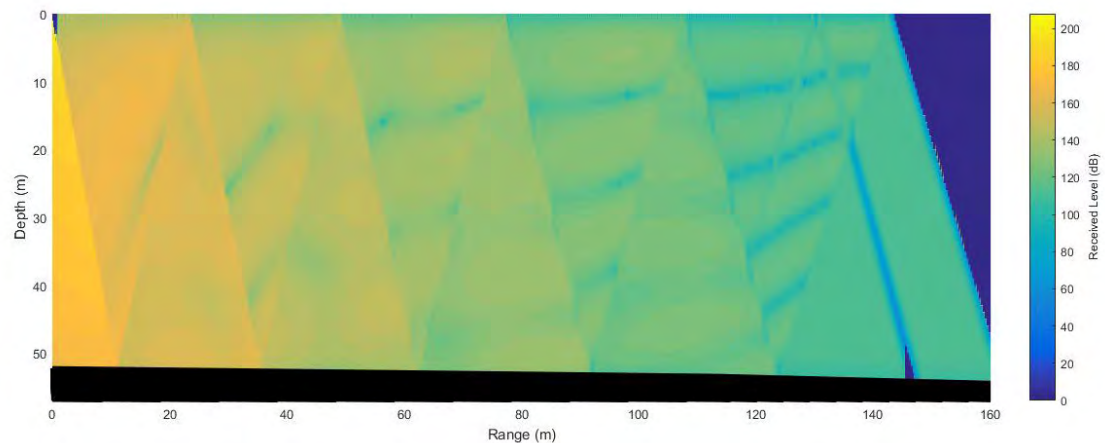
Figure 3-3 BH results during summer months for a chirper; received sound field for a depth/range slice at location 1. Bathymetry is shown in black.
