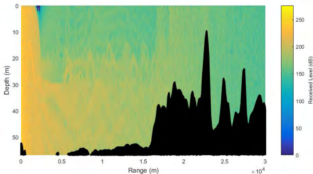
Figure 3-5 BH results during summer months for an UXO; received sound field for a depth/range slice at location 1. Bathymetry is shown in black.
