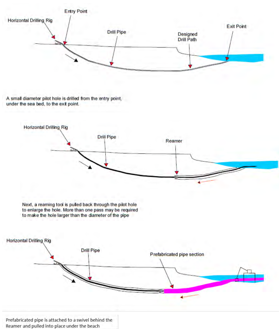
Figure 3-3 Typical HDD
