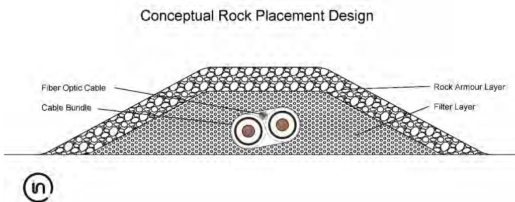
Figure 1-2 Conceptual Rock Placement Design
