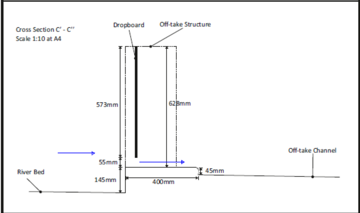
Cross Section of Impoundment Structure & HEP Off-take Structure
