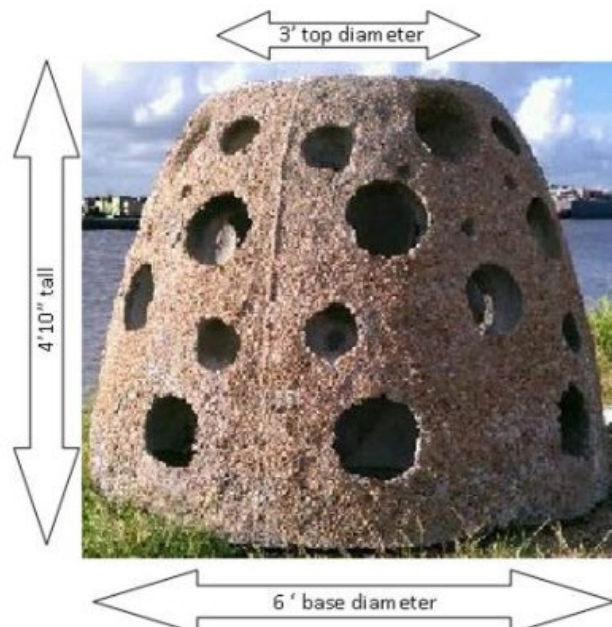
Figure 2-3 Example of a Goliath Reef Ball Module
