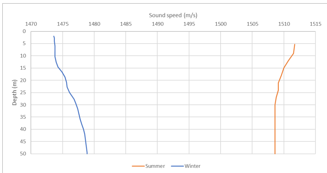
Figure 3-2 Summer and Winter sound speed profiles
