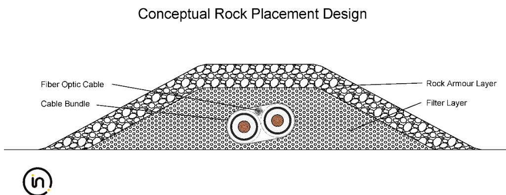
Figure 1-2 Conceptual Rock Placement Design
