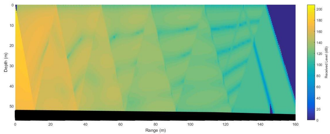
Figure 3-4 BH results during summer months for a multi-beam echosounder; received sound field for a depth/range slice at location 1. Bathymetry is shown in black.
