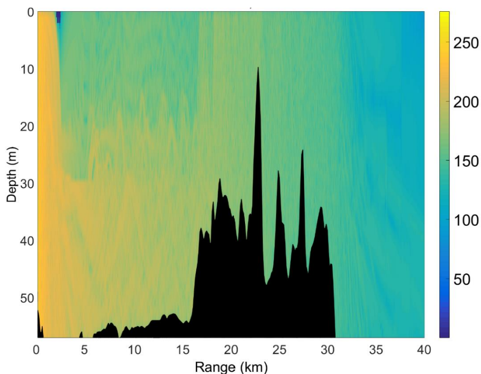
Figure 3-6 BH results during winter months for an UXO at 40kHz; received sound field for a depth/range slice at location 1. Bathymetry is shown in black.
