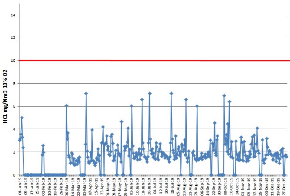
Kiln Main Stack Hydrogen Chloride (ELV 10mg/Nm3)
