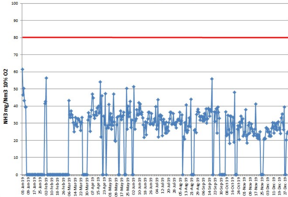
Kiln Main Stack Ammonia (ELV 80mg/Nm3)
