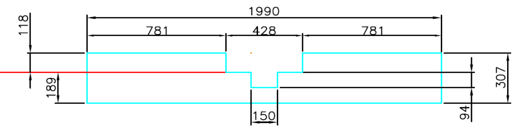
WEIR PLATE 70/30% SHARE (SCALE 1:10)
