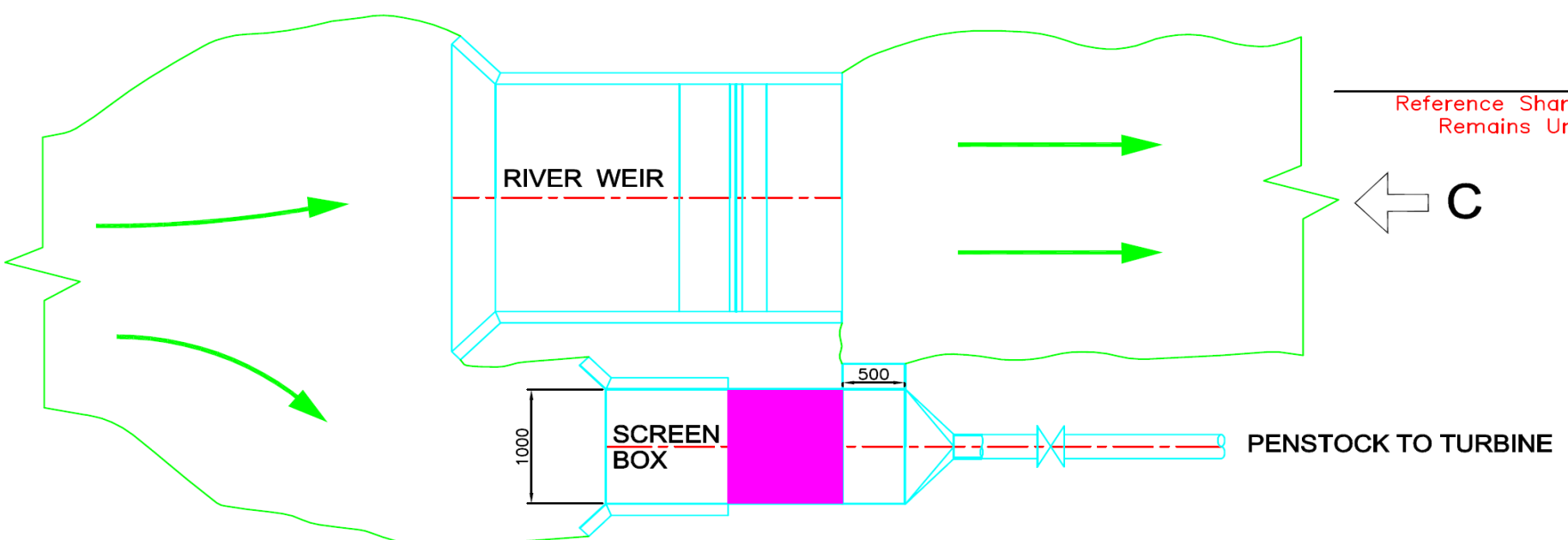
SITE PLAN
