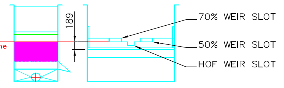
TURBINE WEIR RIVER WEIR WITH HOF AND 50 & 70% WEIR SLOTS
