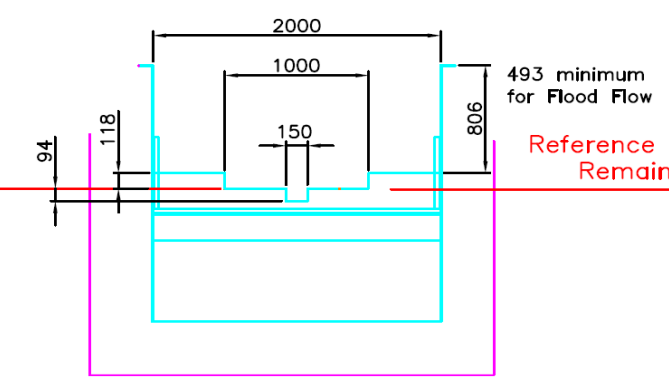
VIEW ON ARROW 'B' (50/50% WEIR PLATE)
