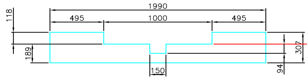
WEIR PLATE 50/50% SHARE (SCALE 1:10)
