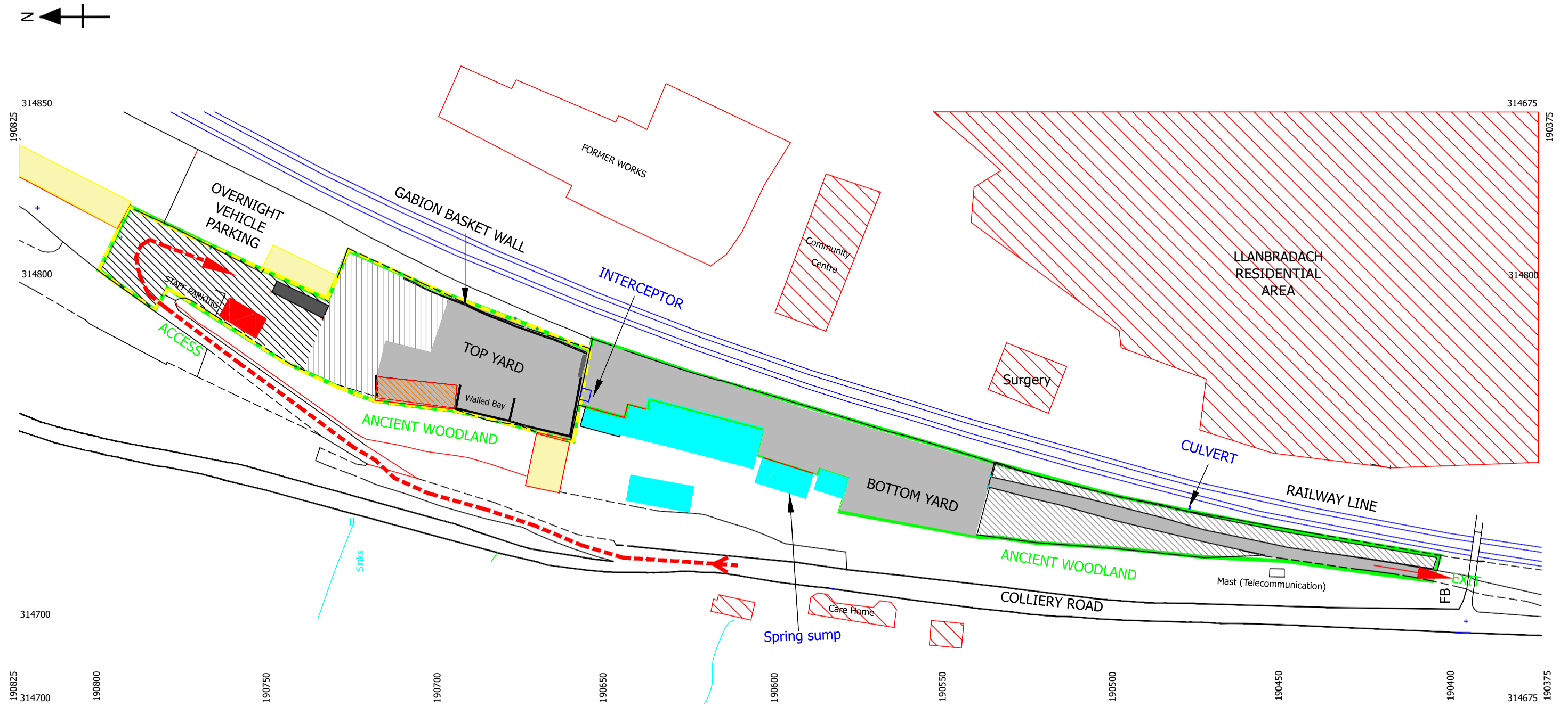
Figure 2 Site Plan
