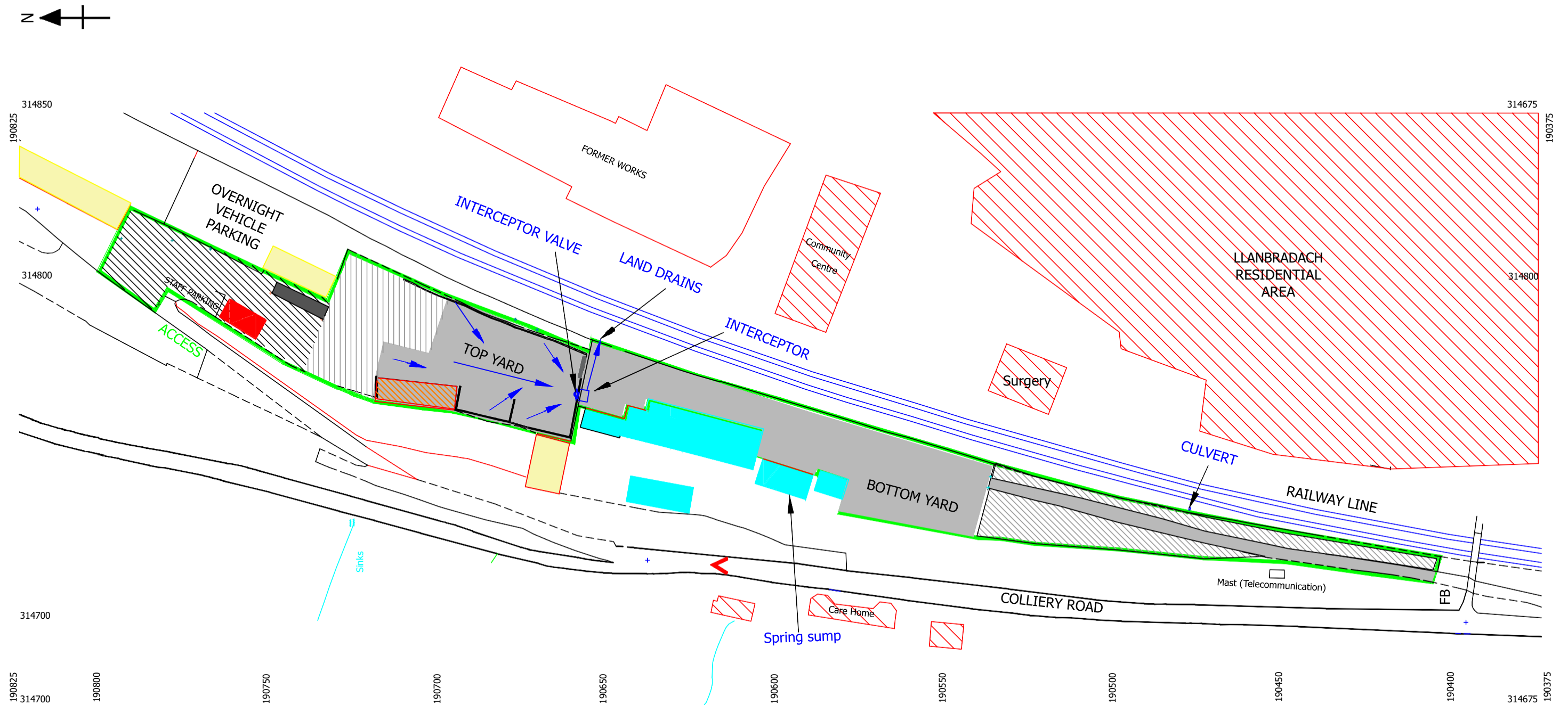
Figure 4 Site Drainage
