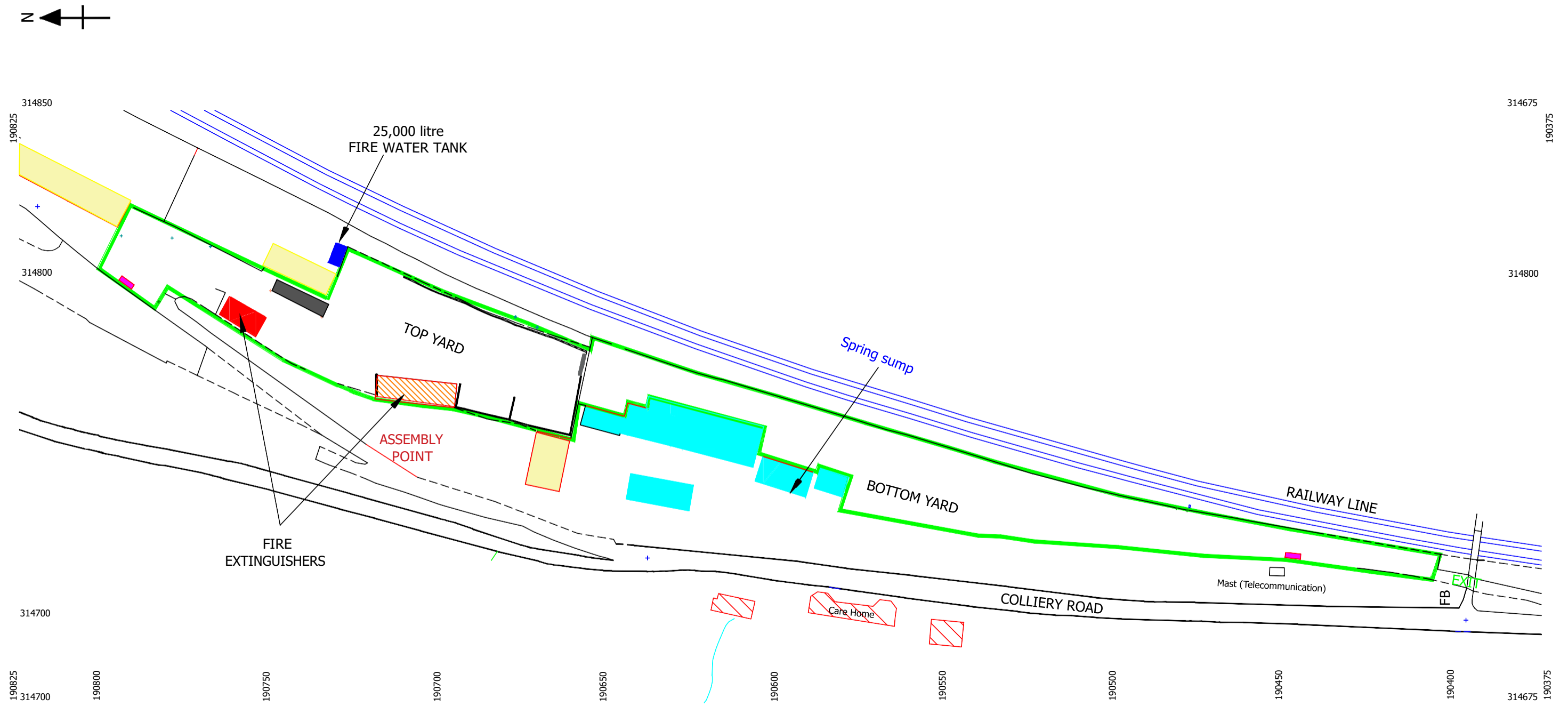
Figure 8 Fire Water and Extinguisher Locations
