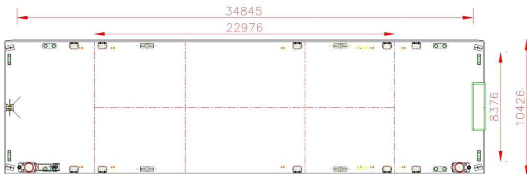
DECK PLAN
