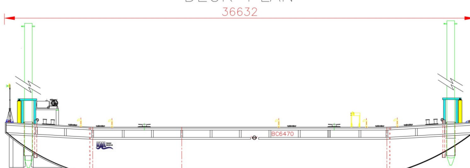
STARBOARD ELEVATION
