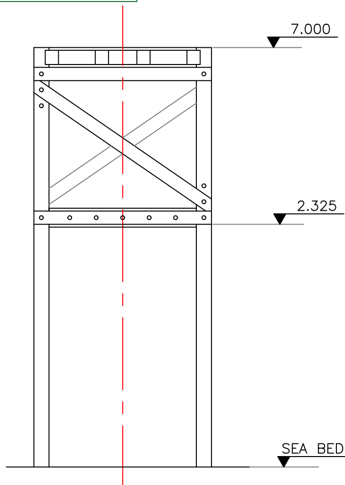
SOUTH ELEVATION
