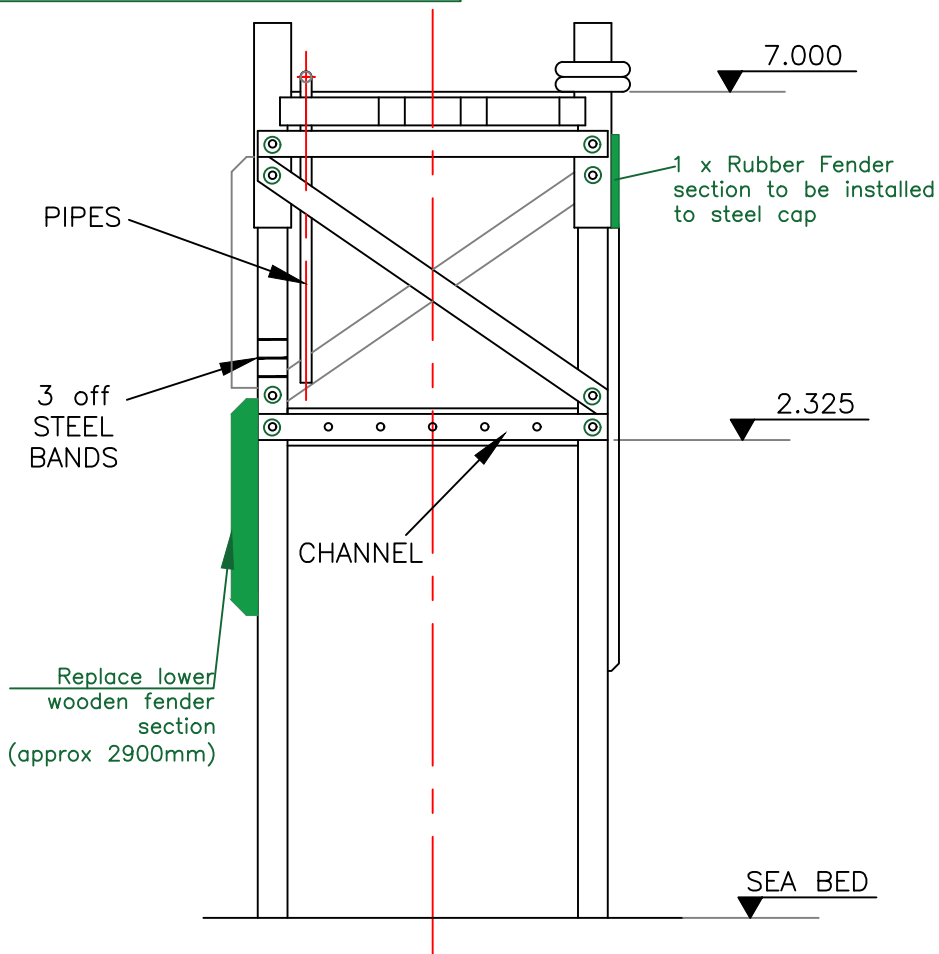
SOUTH ELEVATION
