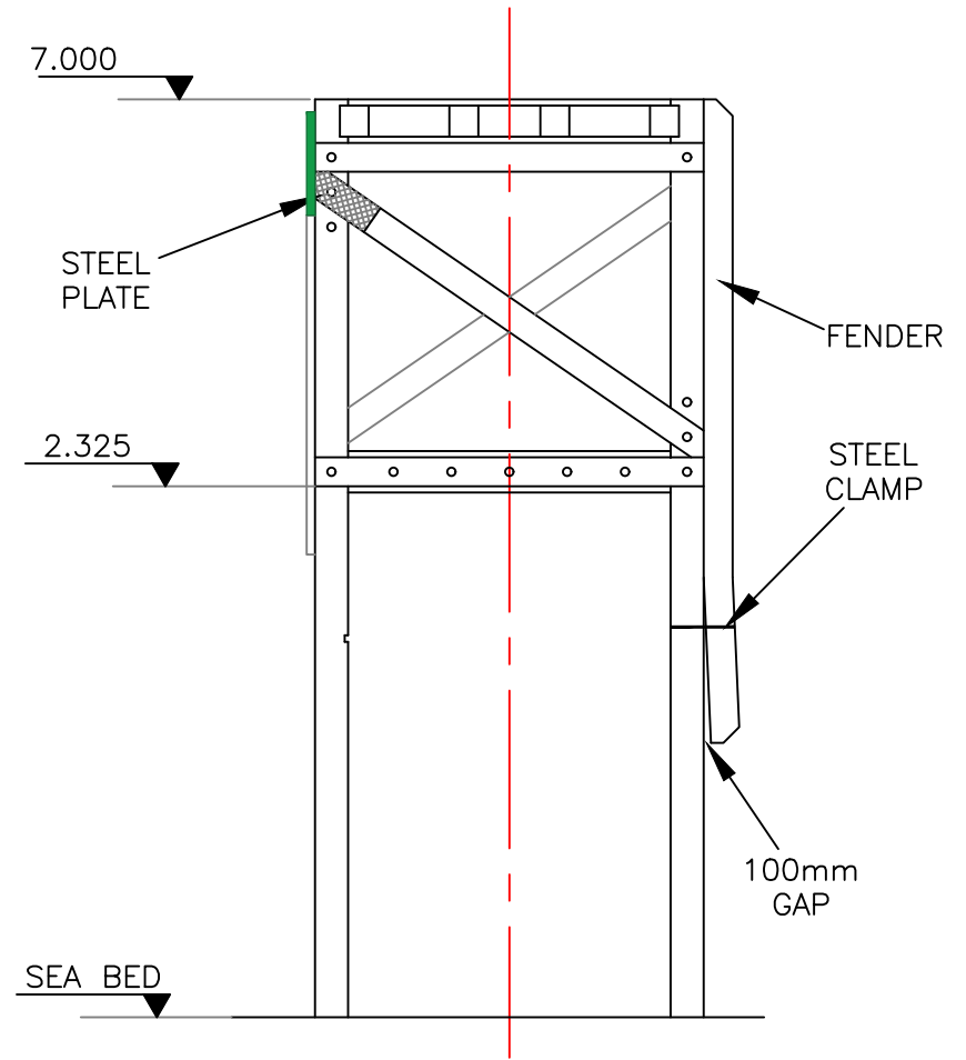
NORTH ELEVATION
