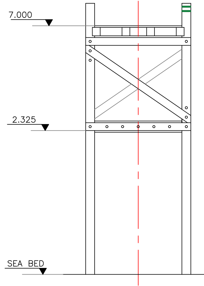
NORTH ELEVATION
