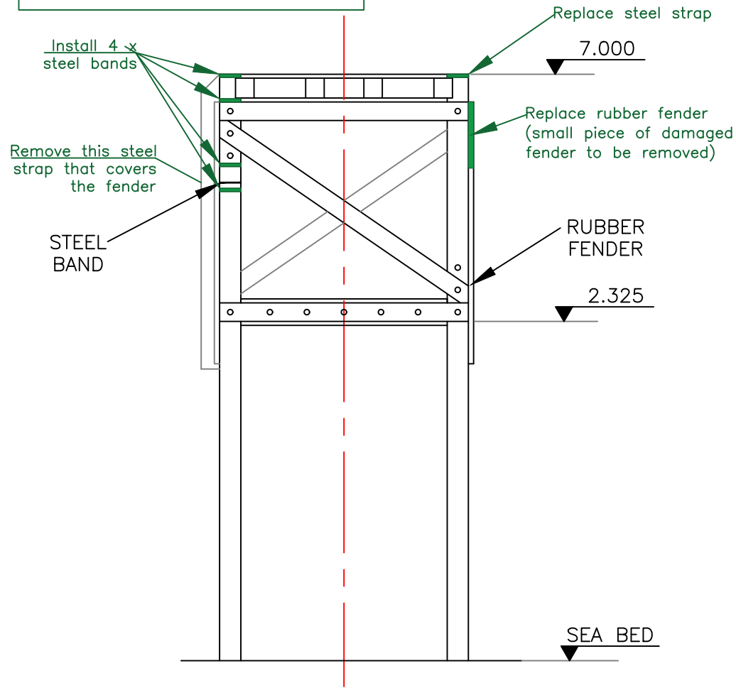
SOUTH ELEVATION
