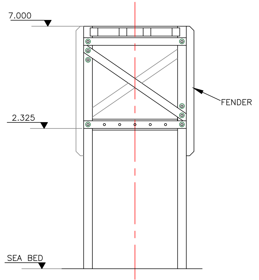
NORTH ELEVATION
