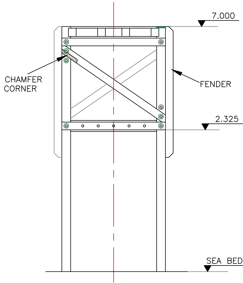
SOUTH ELEVATION
