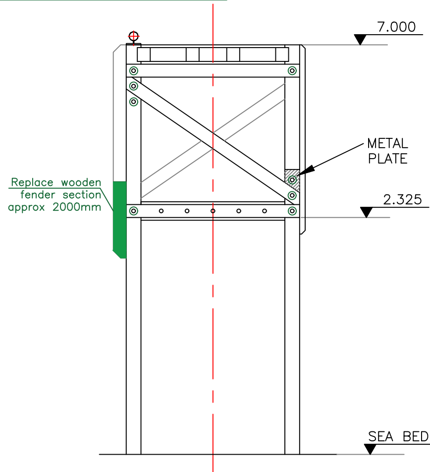
SOUTH ELEVATION
