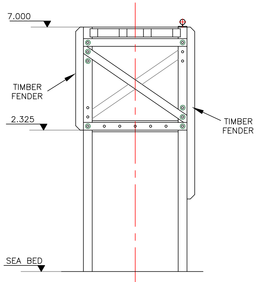
NORTH ELEVATION
