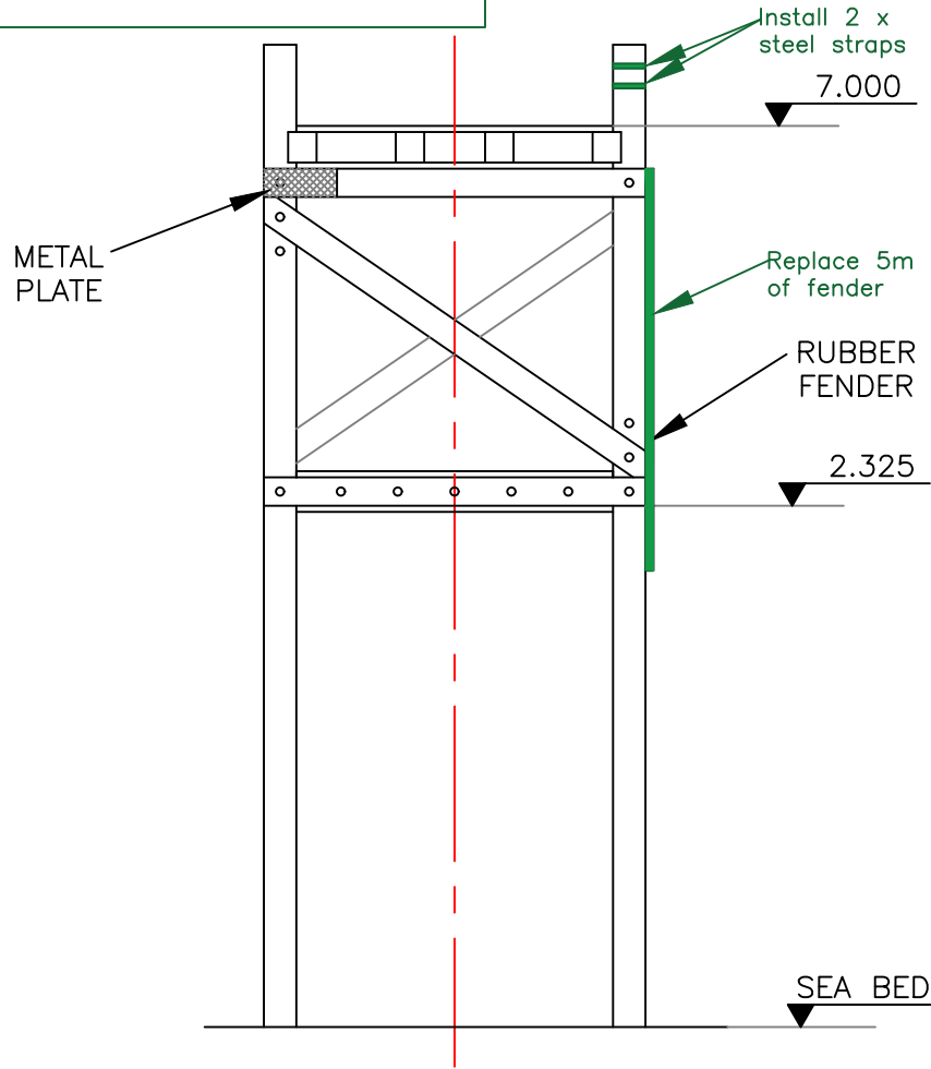
SOUTH ELEVATION
