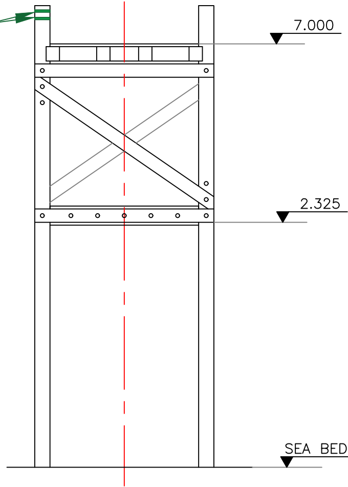
SOUTH ELEVATION
