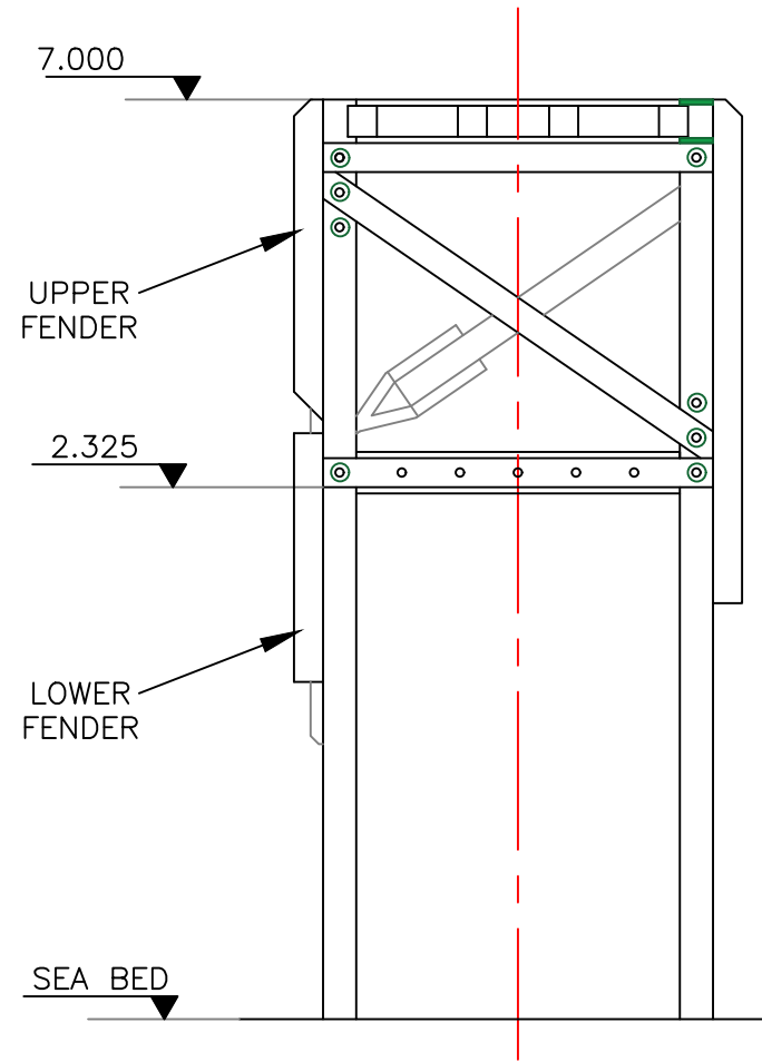
NORTH ELEVATION
