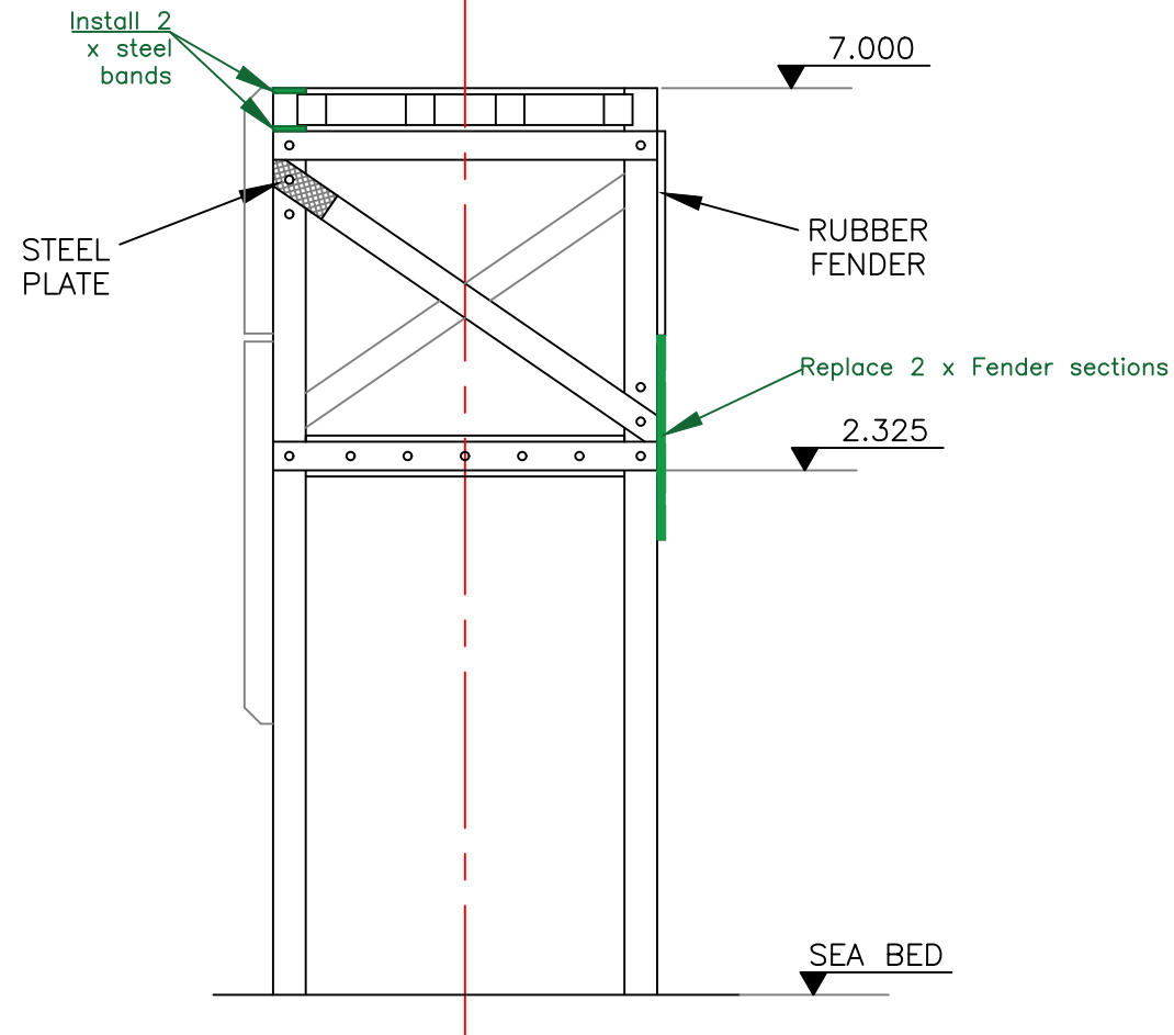
SOUTH ELEVATION
