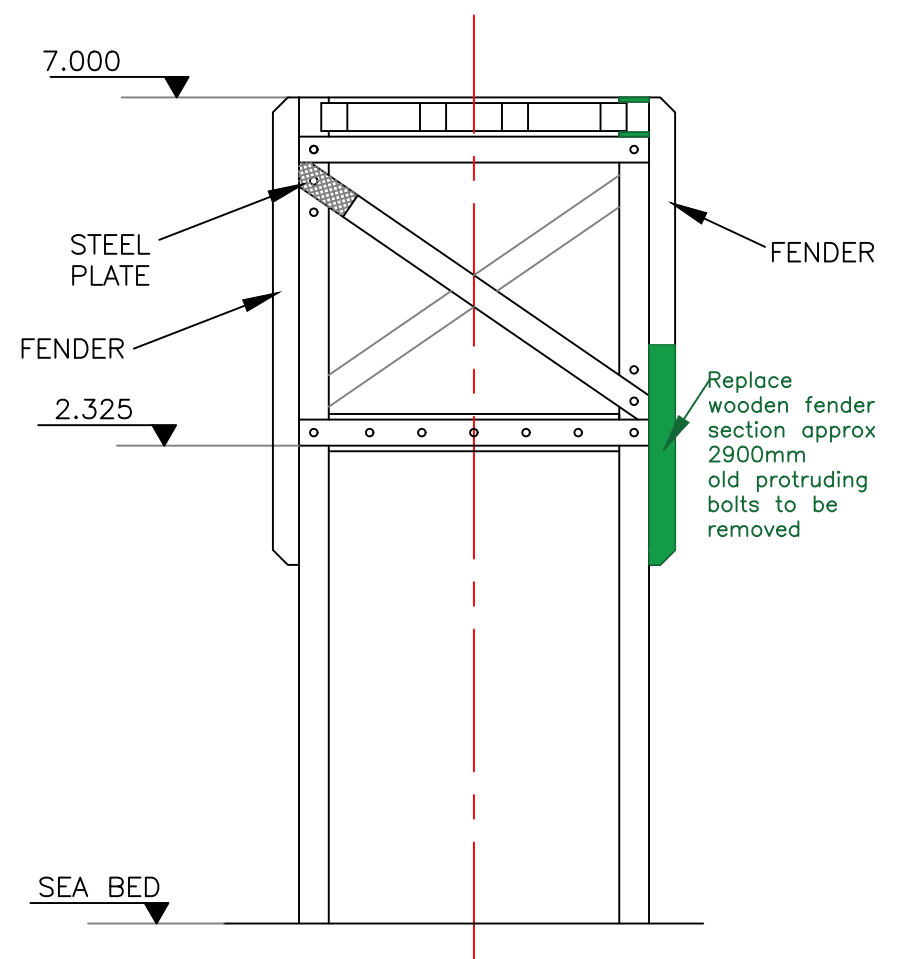
NORTH ELEVATION
