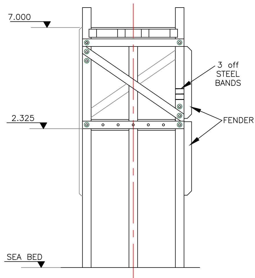
NORTH ELEVATION
