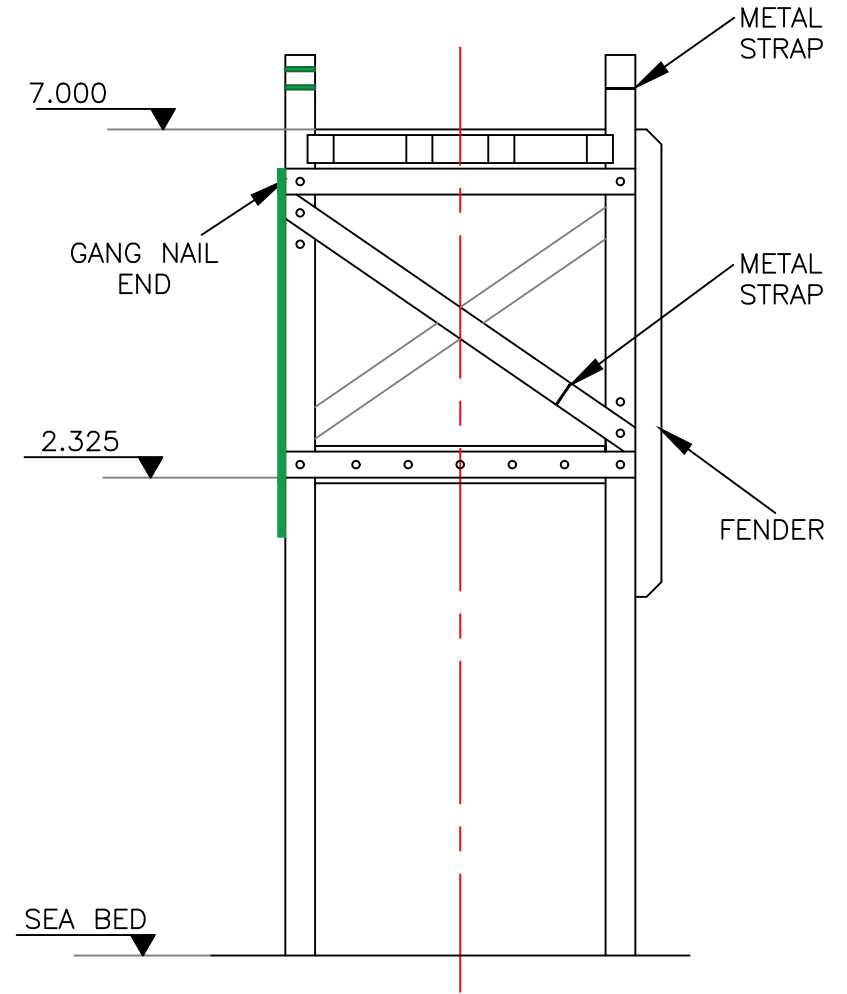
NORTH ELEVATION
