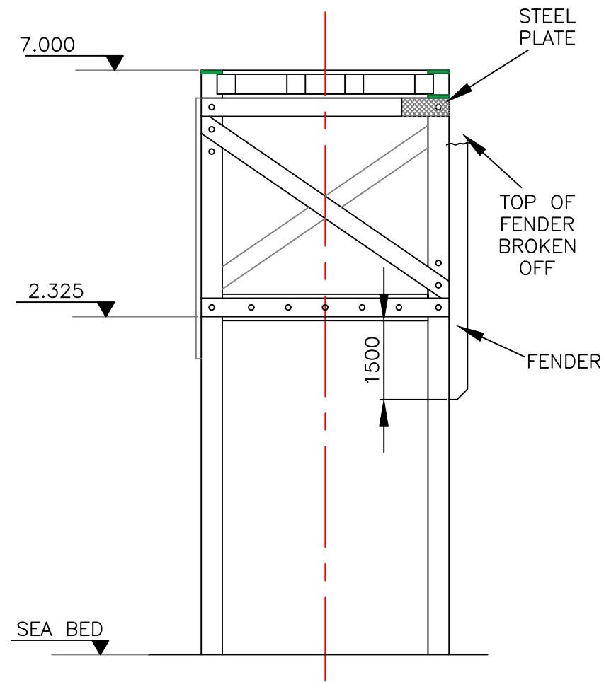
NORTH ELEVATION
