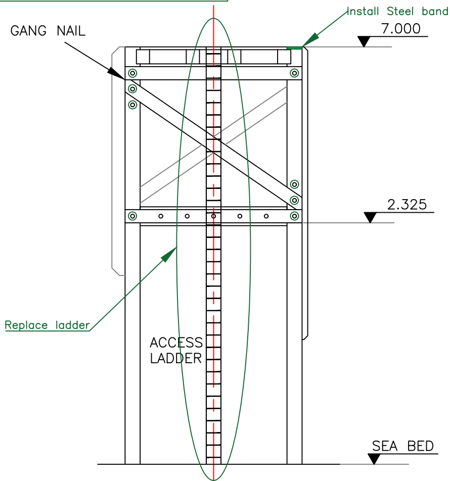
SOUTH ELEVATION
