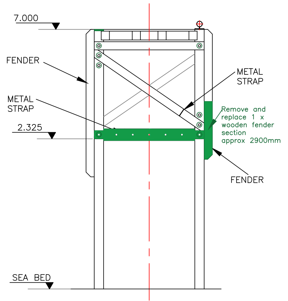
NORTH ELEVATION
