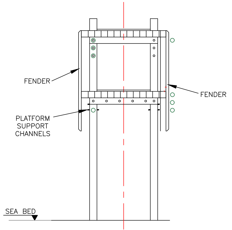
NORTH ELEVATION
