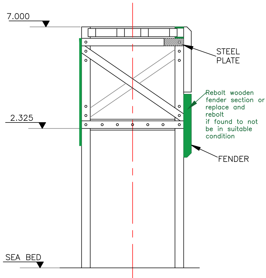
NORTH ELEVATION
