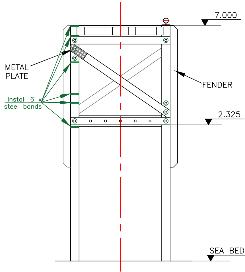
SOUTH ELEVATION
