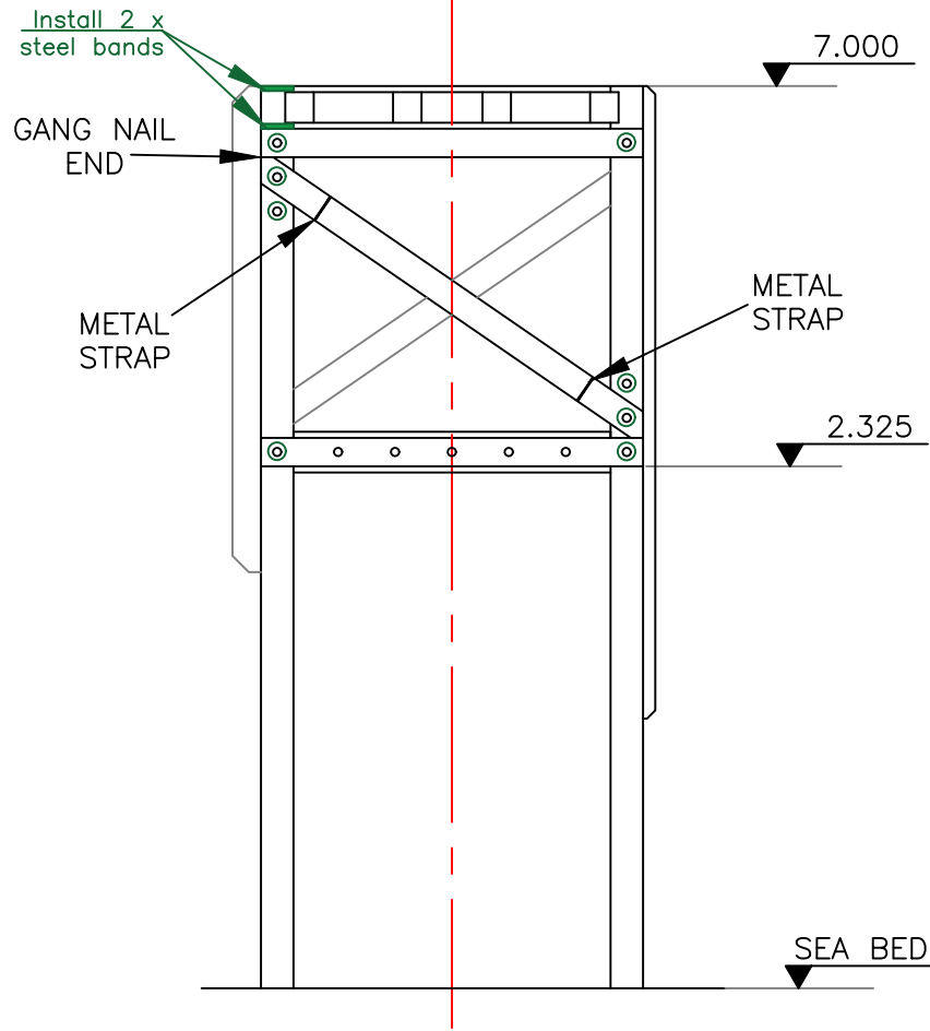
SOUTH ELEVATION
