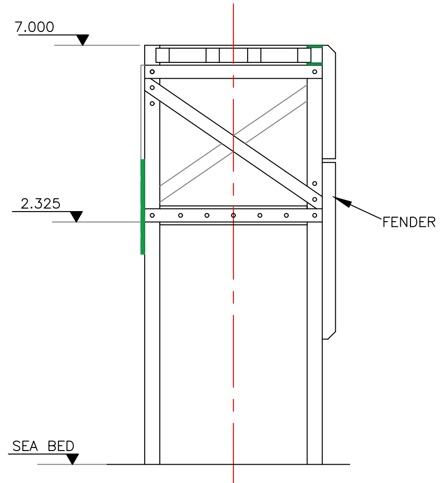
NORTH ELEVATION
