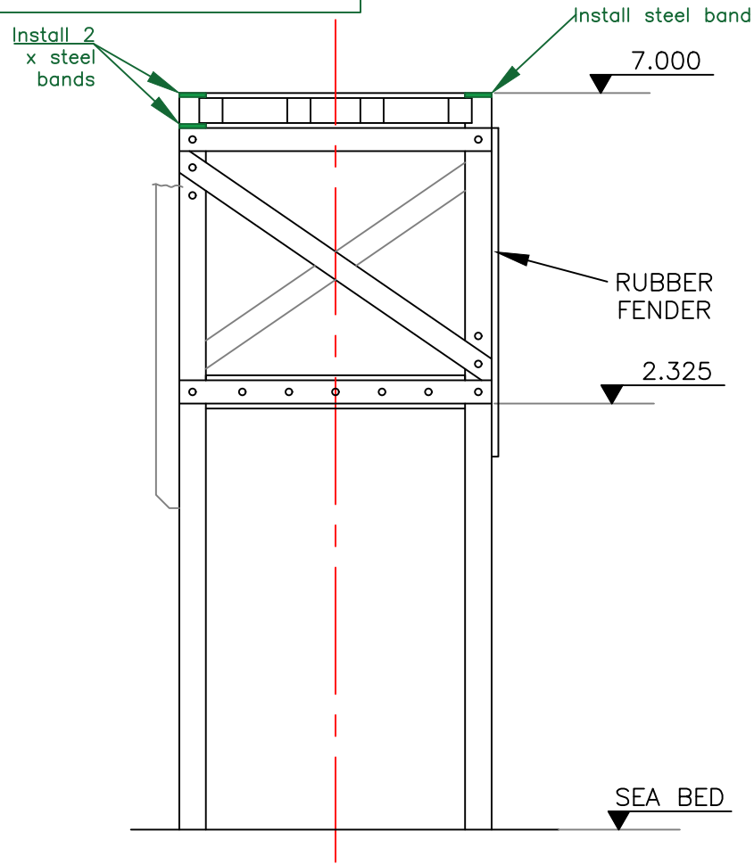
SOUTH ELEVATION
