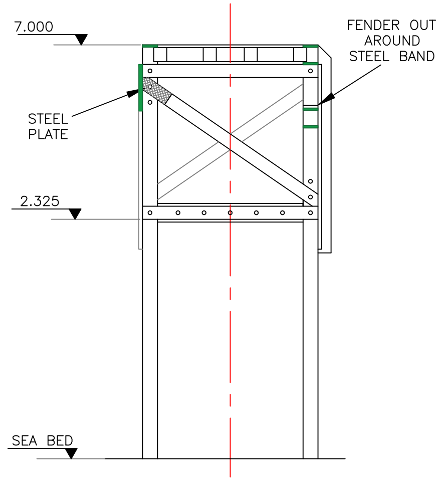
NORTH ELEVATION
