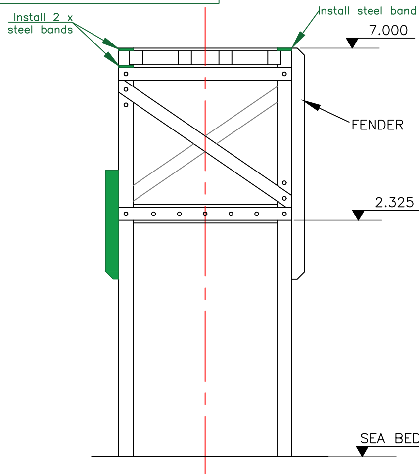
SOUTH ELEVATION
