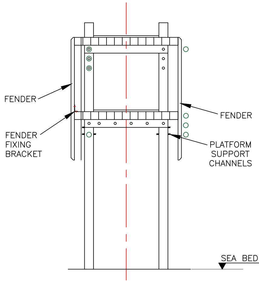
SOUTH ELEVATION
