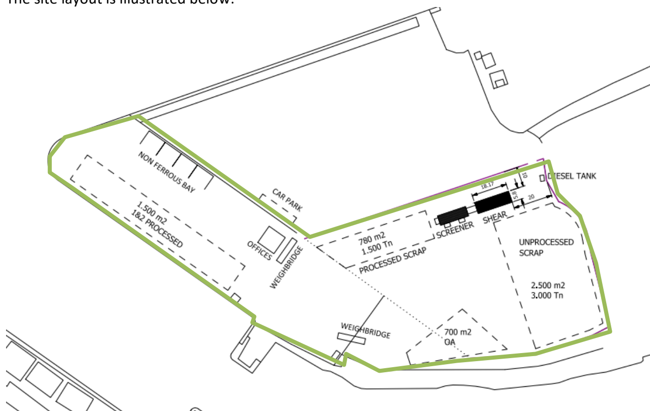
Figure 2 – Site layout
