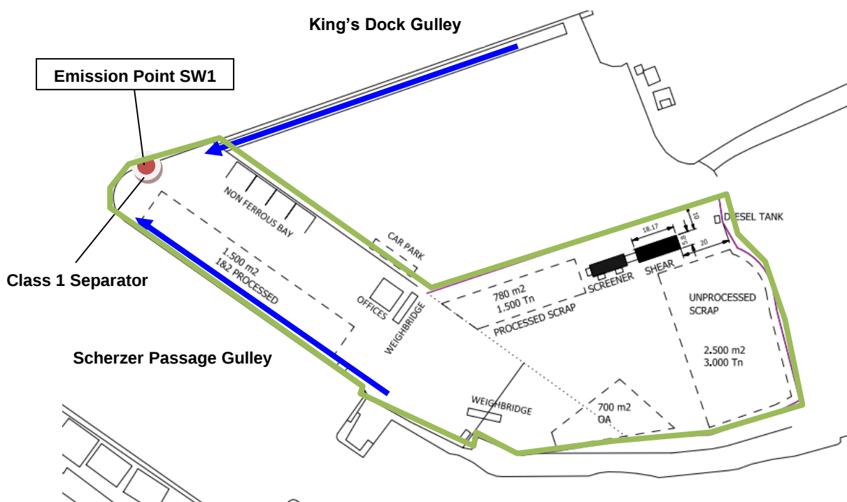
Figure 3 – Site Drainage
