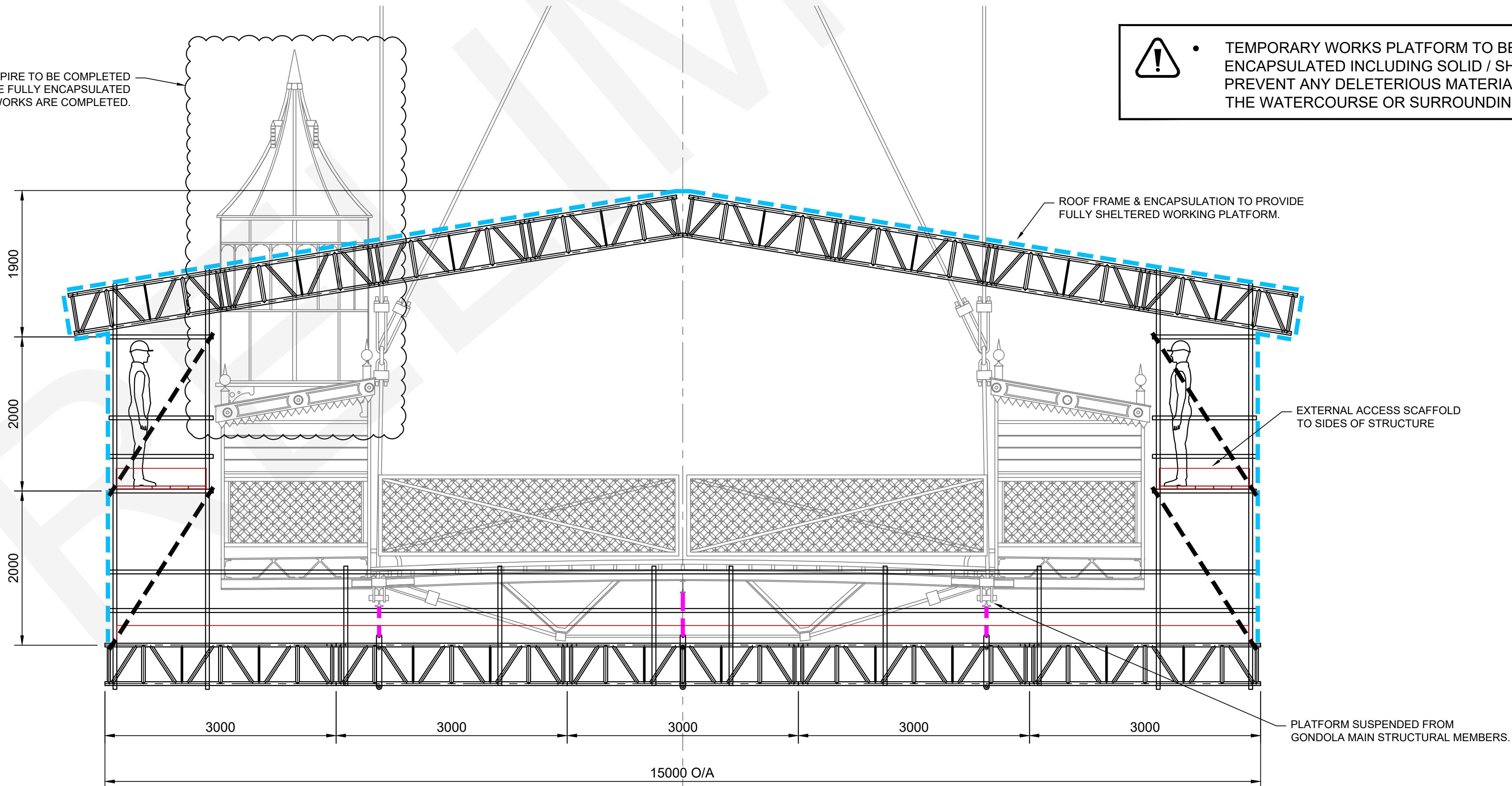
END ELEVATION (SCALE 1:40)
