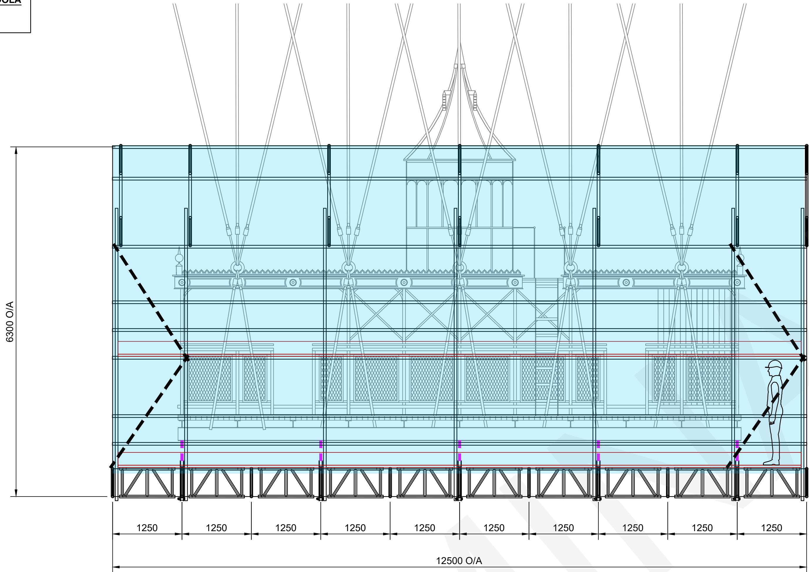
SIDE ELEVATION (SCALE 1:40)
