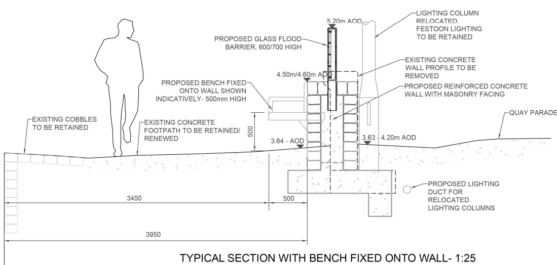
TYPICAL SECTION WITH BENCH FIXED ONTO WALL- 1:25
