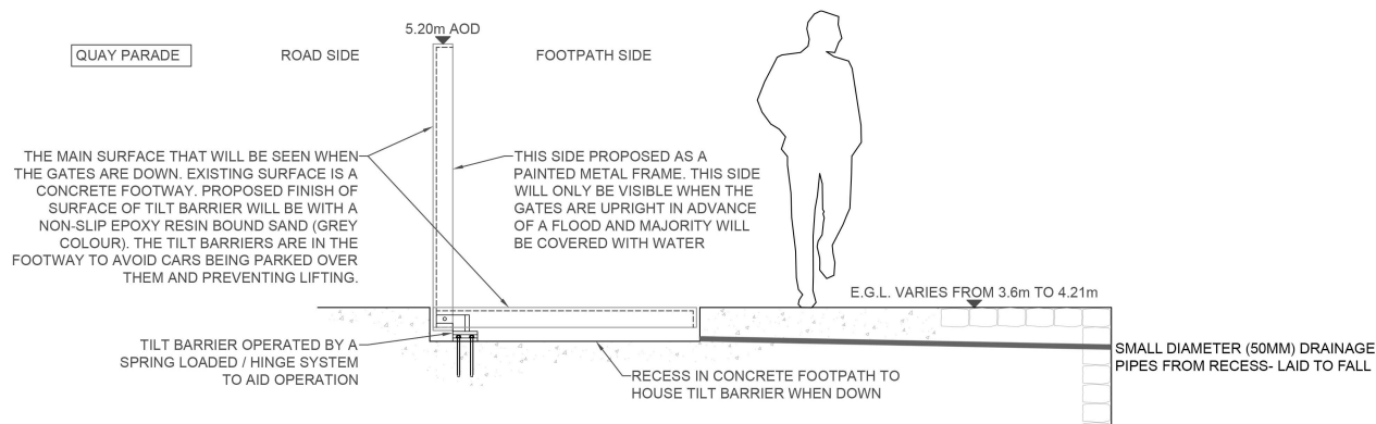
TYPICAL TILT BARRIER DETAIL- 1:25
