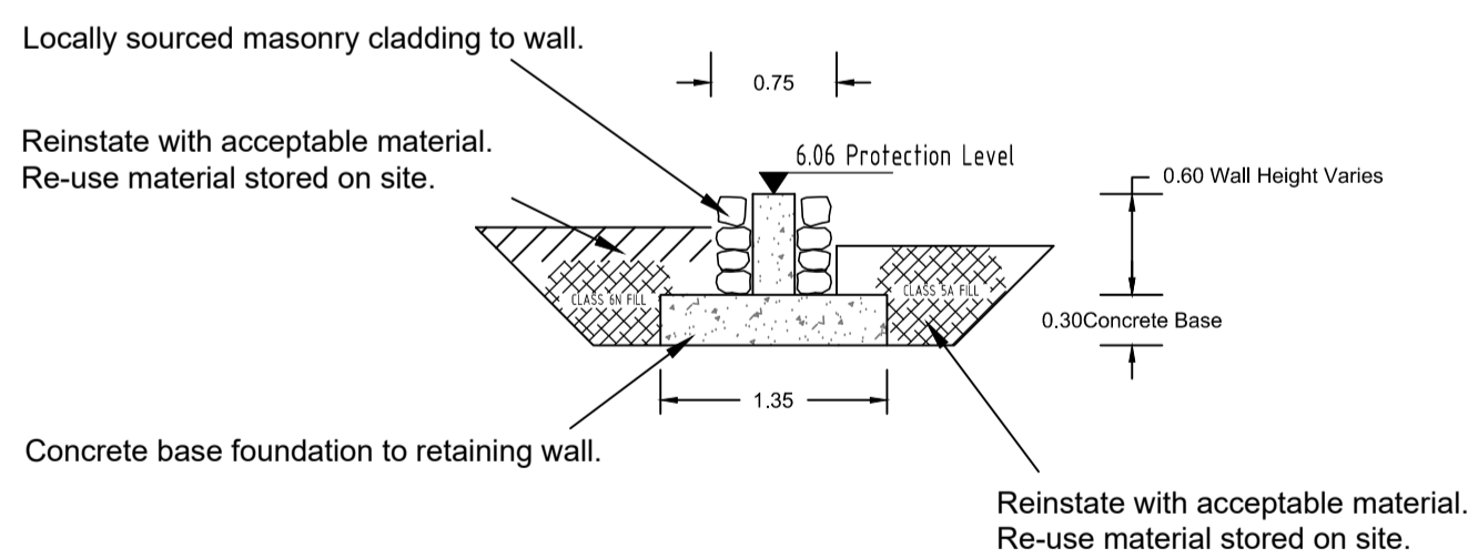
Typical Section Showing Wall Type A Details. Scale 1:50
