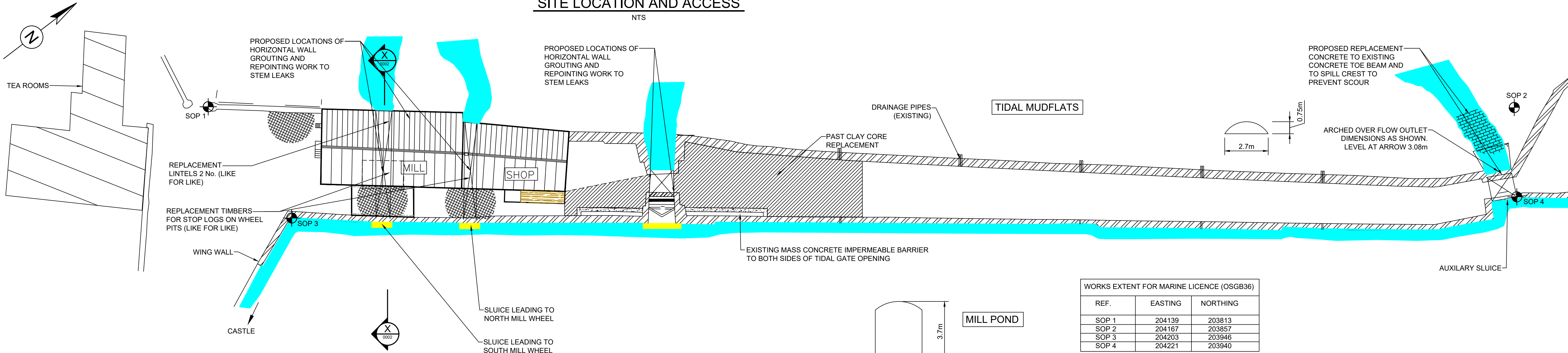
PLAN OF CAUSEWAY SHOWING REPAIR ITEMS
