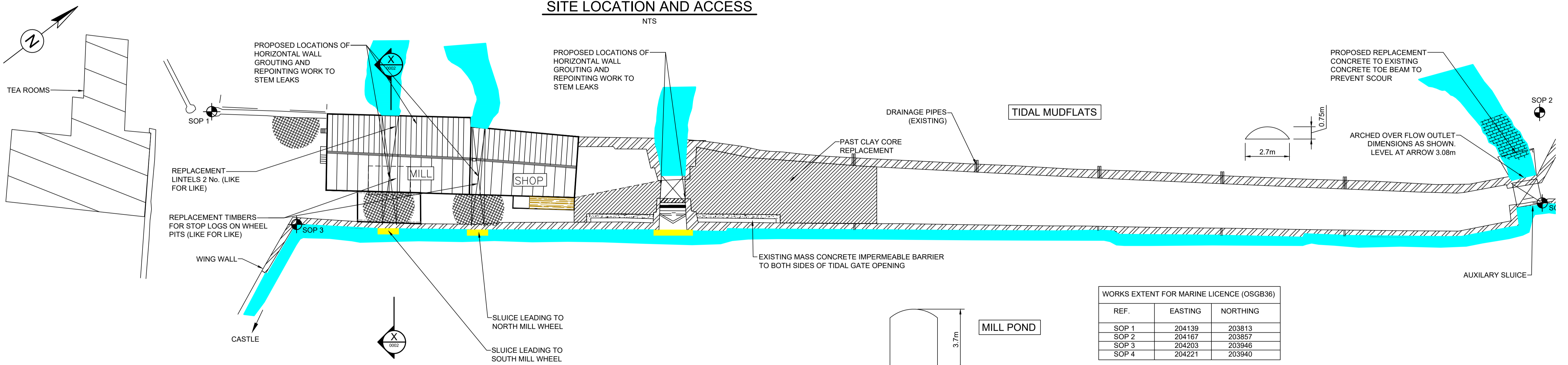
PLAN OF CAUSEWAY SHOWING REPAIR ITEMS 1:250
