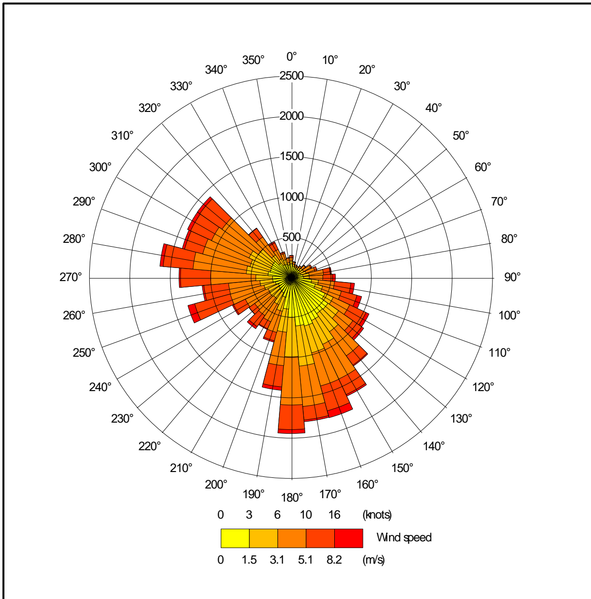
Figure 3e. The wind rose. Derived data from the Trawscoed weather station, 2014-2017
