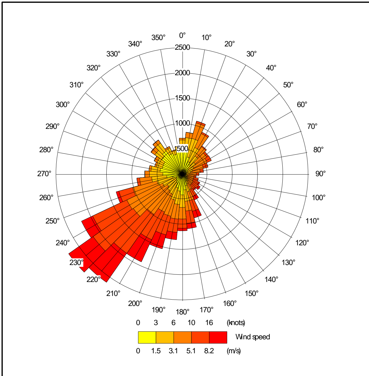
Figure 3c. The wind rose. Derived data from the Sennybridge weather station, 2014-2017
