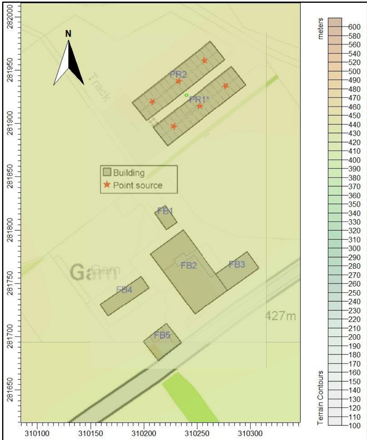
Figure 4. The positions of modelled buildings & sources
