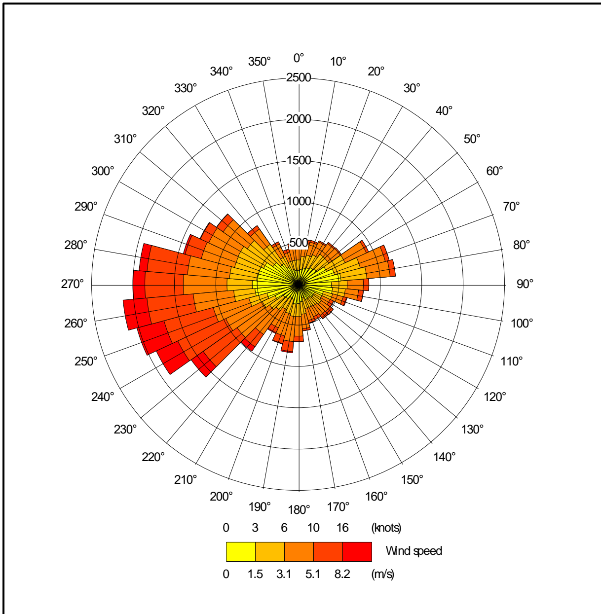
Figure 3d. The wind rose. Derived data from the Shobdon weather station, 2014-2017
