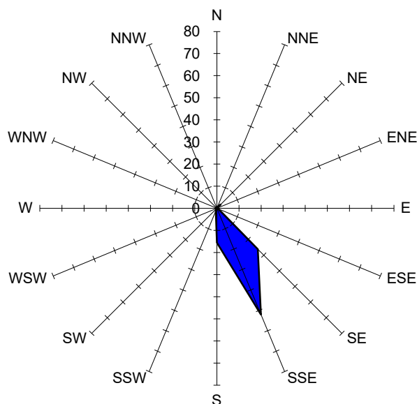
Figure 1: Wind Rose Illustrating Mean Direction from the South Southeast.
