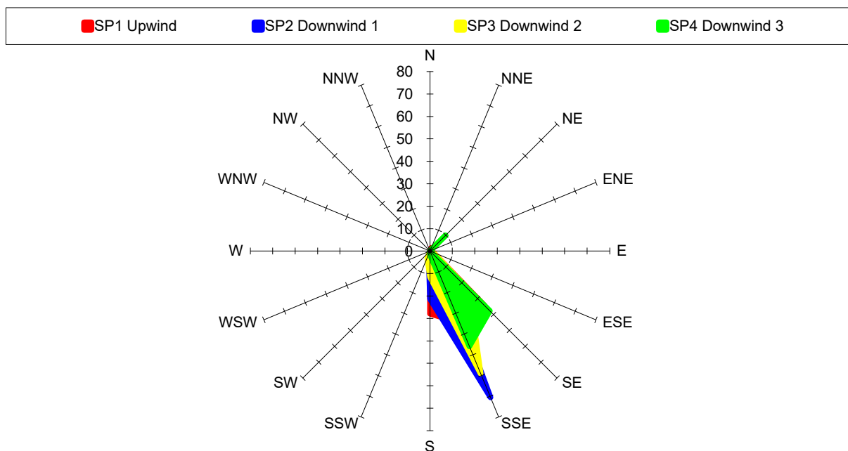
Figure 2: Wind Rose Illustrating Wind Patterns at Sample Locations SP1 - SP4.
