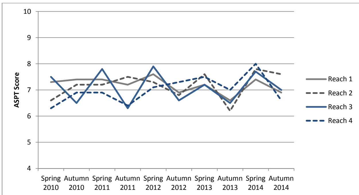
Figure 2: ASPT (Revised) Score - 2010 to 2014
