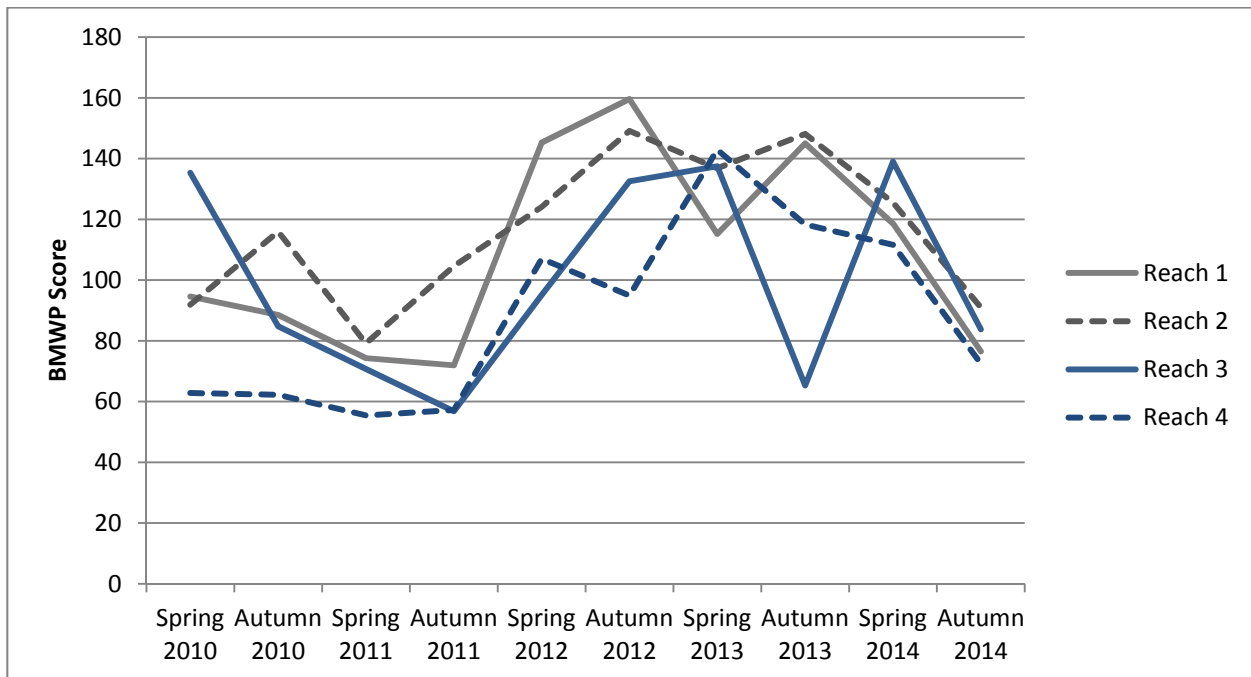
Figure 1: BMWP (Revised) Scores - 2010 to 2014
