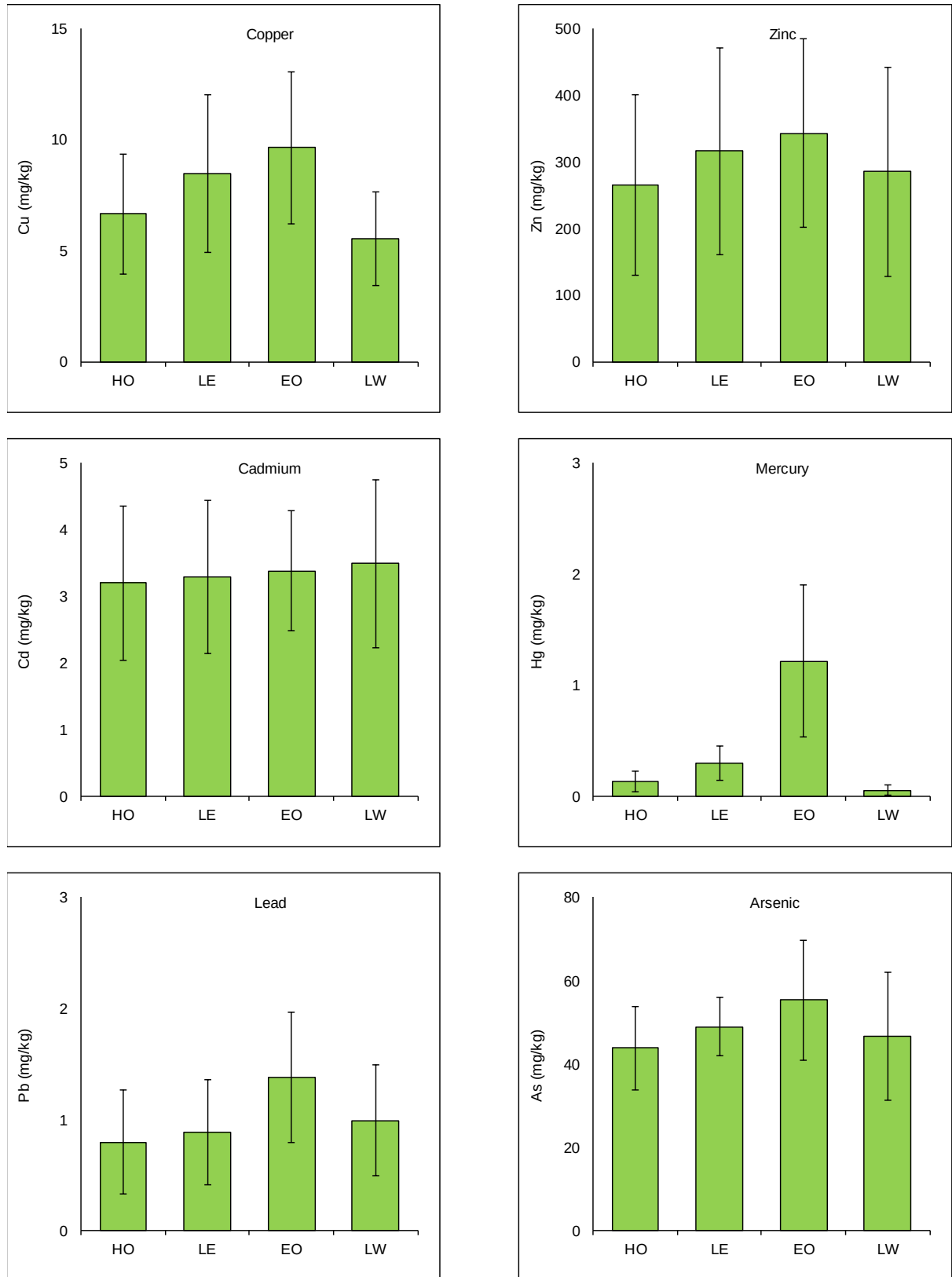
Figure 3.9 : Mean metal concentrations (mg/kg dry weight) in the tissue of the seaweed Fucus serratus averaged between 2010 and 2016 at sites sampled in 2016. Error bars represent standard deviation.
