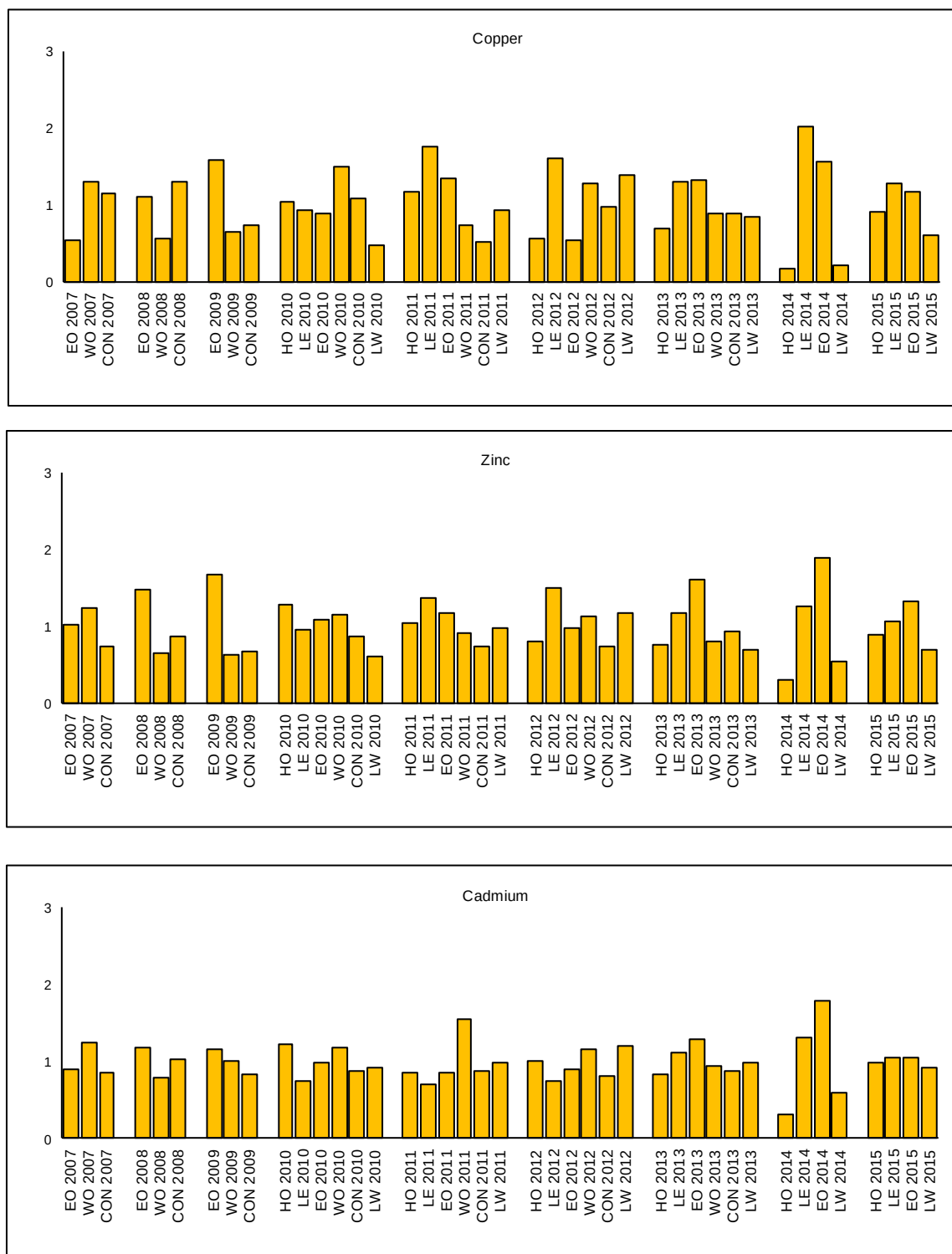
Figure 3.2 : Standardised metal concentrations (SM) in the tissue of the dogwhelk Nucella lapillus at each site in each year (sites CON and WO sampled 2007 – 2013 only, data not available for 2016).
