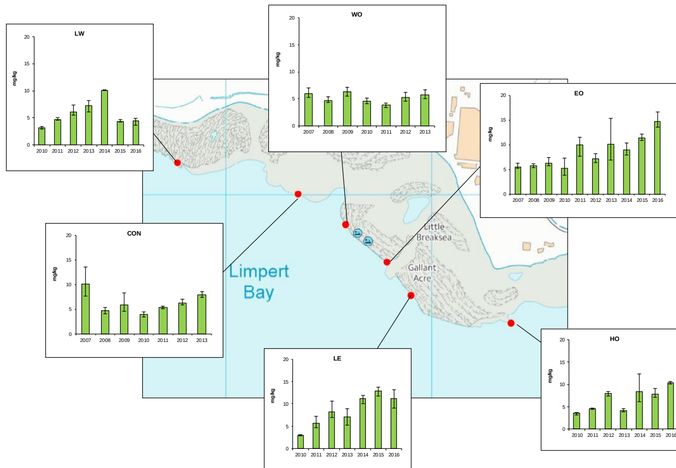
Figure 3.7 : Mean concentrations (mg/kg dry weight) of metals in the tissue of the seaweed Fucus serratus at each site. Error bars represent individual replicate concentration range (Sites CON and WO sampled 2007-2013 only): (i) Copper;
