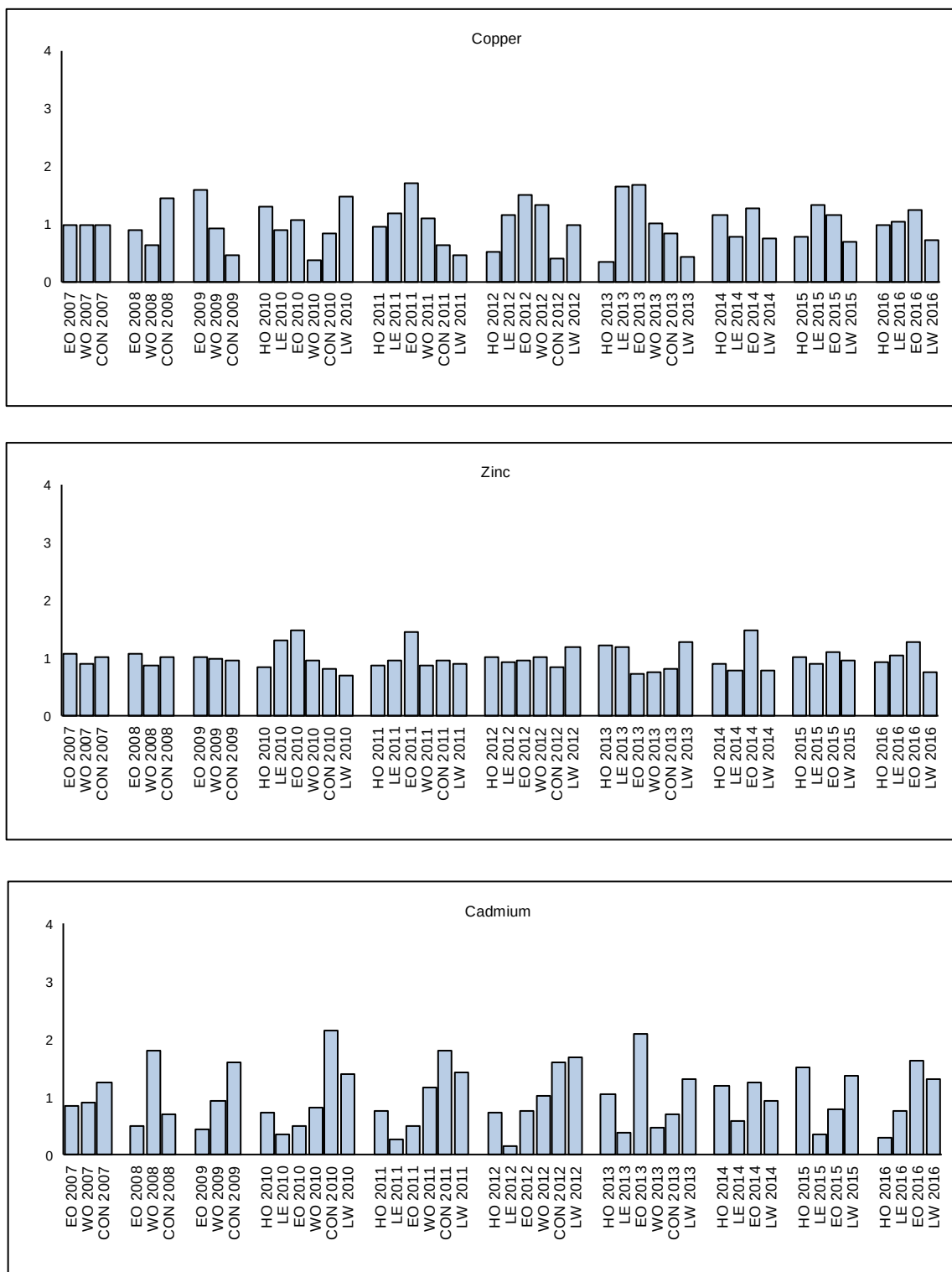
Figure 3.5 : Standardised metal concentrations in the tissue of the limpet Patella vulgata at each site in each year. (Sites CON and WO sampled 2007-2013 only).
