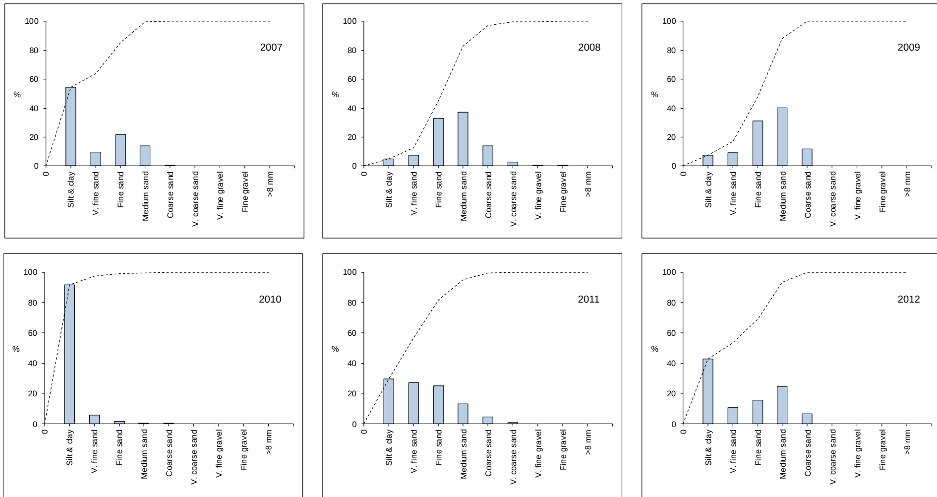
Figure 3.11 : Mean size-frequency histogram (bar) and cumulative frequency (line) plot for sediment granulometric data from the Aberthaw sediment site between 2007 and 2016 (n= 5).
