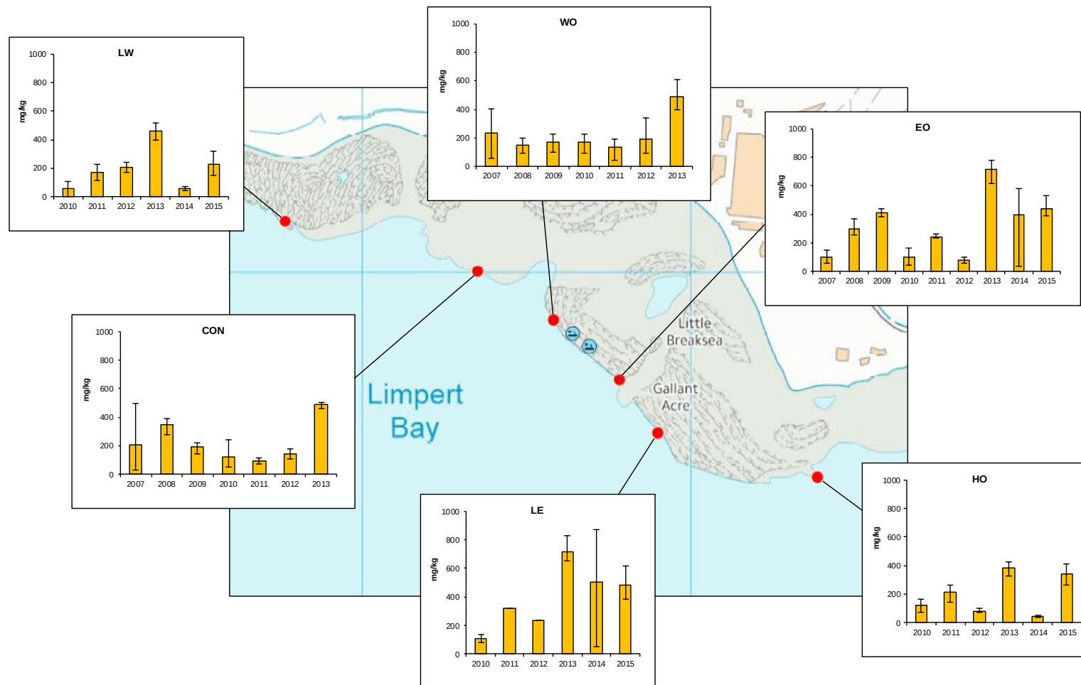
Figure 3.1 : Mean concentrations (mg/kg dry weight) of metals in the tissue of the dogwhelk Nucella lapillus at each site. Data not available for 2016. (Sites CON and WO sampled 2007-2013 only) Error bars represent individual replicate concentration range: (i) Copper;
