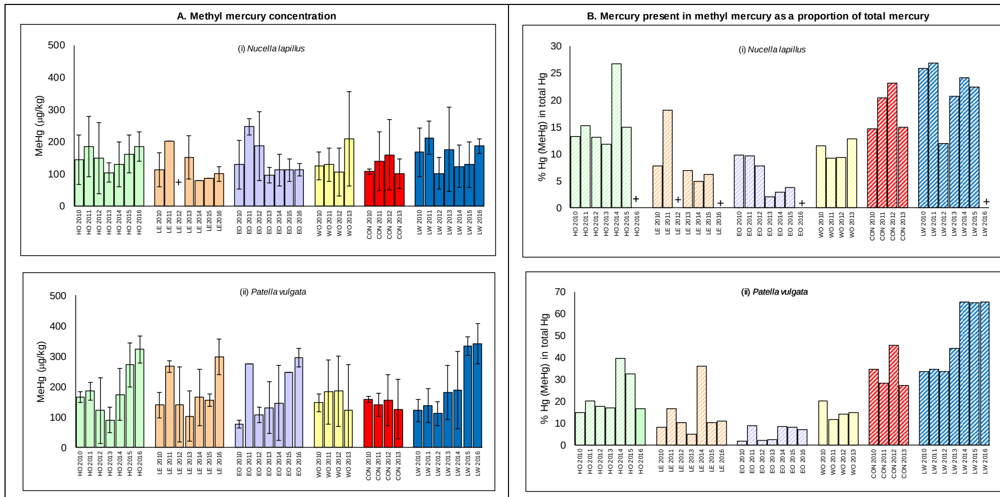
Figure 3.10 : Mean methyl mercury (MeHg) concentration ( \mu\text{g/kg} dry weight) in Nucella lapillus and Patella vulgata 2010 - 2016. Error bars represent standard deviation; + = no data. NB: the graphs are approximate as some organic mercury may be converted into inorganic mercury during the analytical process and therefore be included in the inorganic result (however, it is probable that most of it will not be included in the inorganic result).
