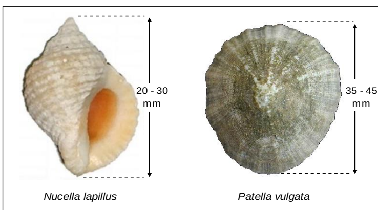
Figure 2.2 : Standard size range for dogwhelk ( Nucella lapillus ) and limpet ( Patella vulgata ).
