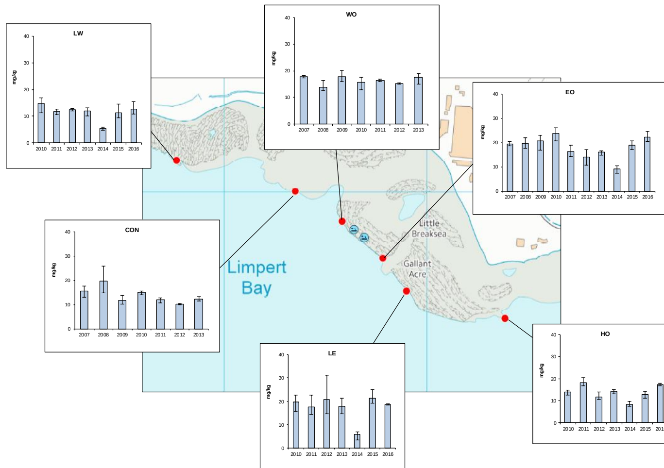
Figure 3.4 : Mean concentrations (mg/kg dry weight) of metals in the tissue of the limpet Patella vulgata at each site. Error bars represent individual replicate concentration range (Sites CON and WO sampled 2007-2013 only): (i) Copper;
