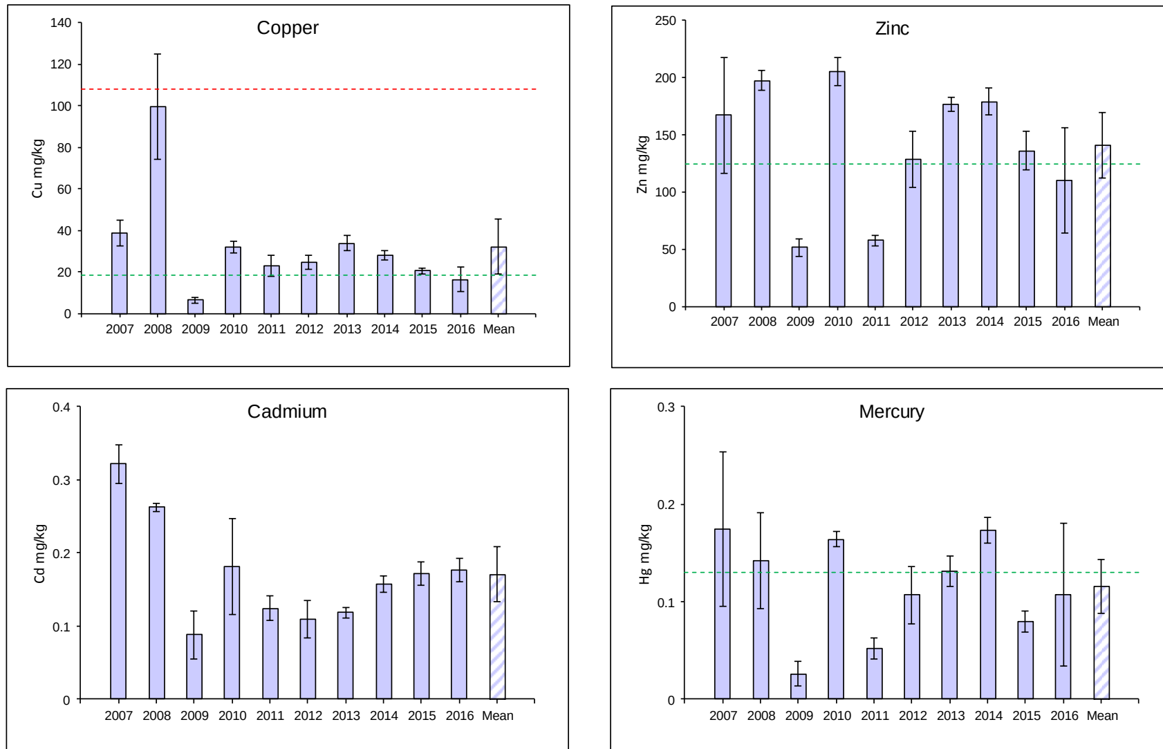
Figure 3.12 : Mean sediment-bound metal concentrations (mg/kg) at the Aberthaw sediment site 2007 – 2016 (n= 5). Error bars represent standard deviation; dotted lines represent TEL (green) and PEL (red). Where a dotted line is missing the TEL and/or PEL is greater than the scale of the graphs.
