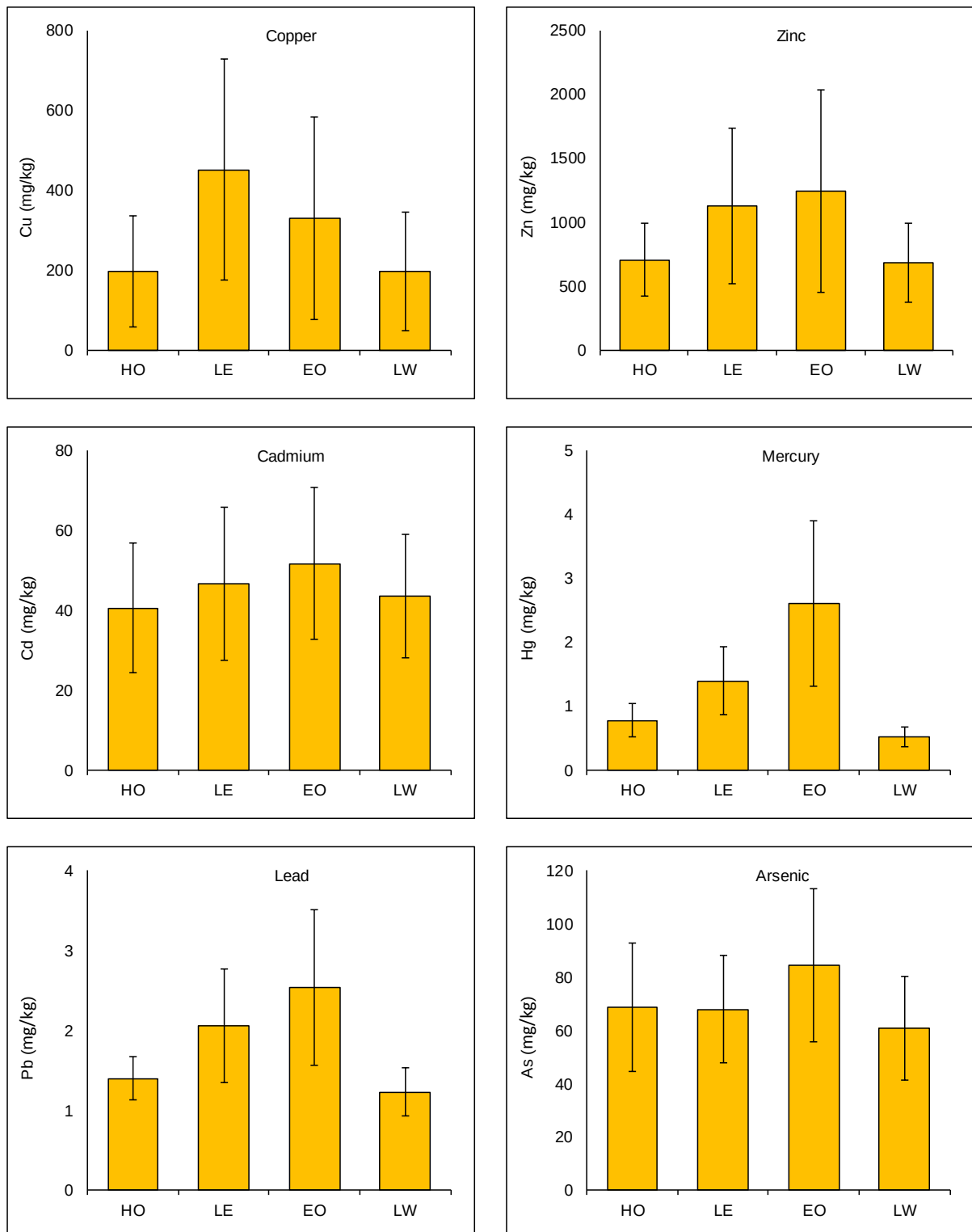
Figure 3.3 : Mean metal concentrations (mg/kg dry weight) in the tissue of the dogwhelk Nucella lapillus averaged between 2010 and 2015 at sites sampled in 2015. Data not available for 2016. Error bars represent standard deviation.
