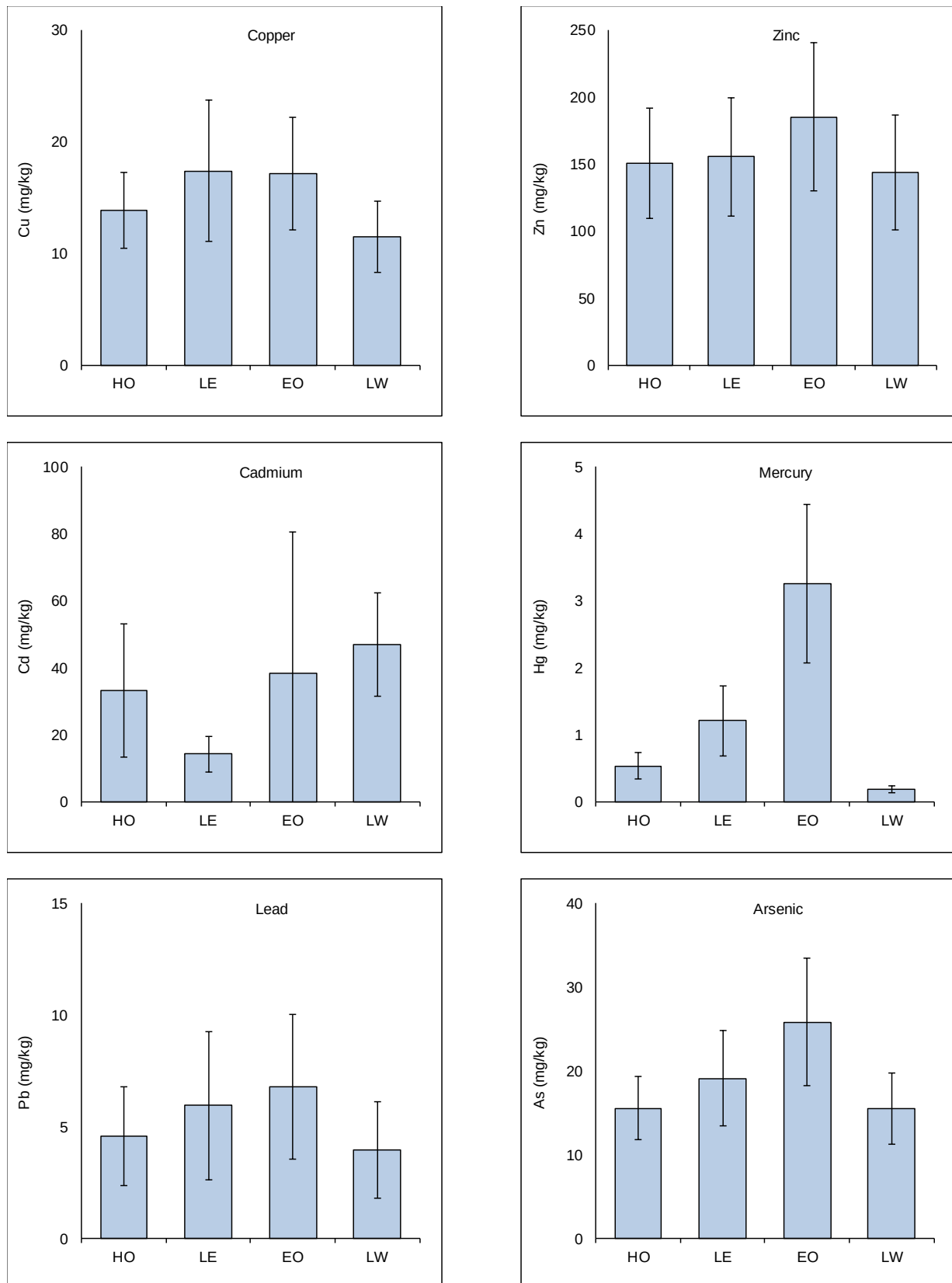
Figure 3.6 : Mean metal concentrations (mg/kg dry weight) in the tissue of the limpet Patella vulgata averaged between 2010 and 2016 at sites sampled in 2016. Error bars represent standard deviation.
