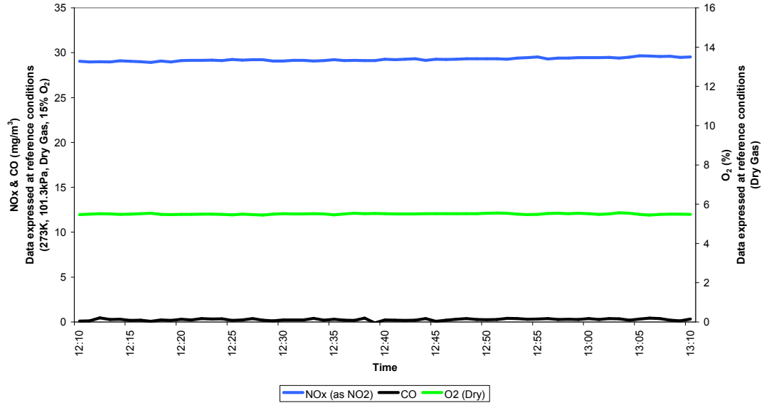
Continuous Emissions Monitoring of Combustion Gases on A4 (MP Fired Boiler 002A) at Cofely (GDF Suez), Dow Corning, Barry on the 1 st September 2014.
