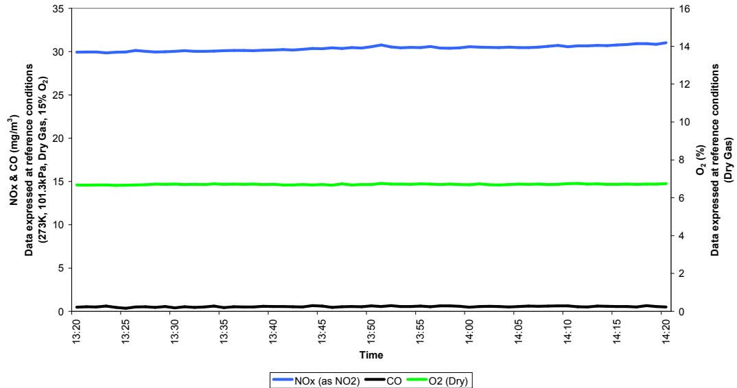
Continuous Emissions Monitoring of Combustion Gases on A5 (MP Fired Boiler 002B) at Cofely (GDF Suez), Dow Corning, Barry on the 1 st September 2014.
