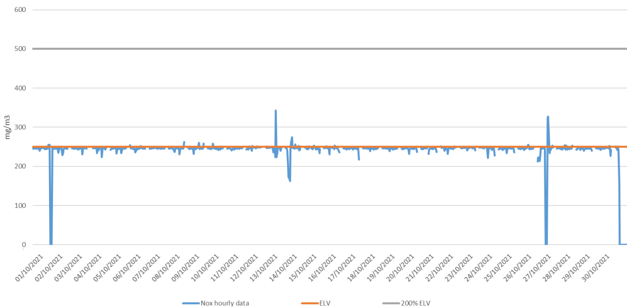
Summary of Nox Emissions - Oct 2021
