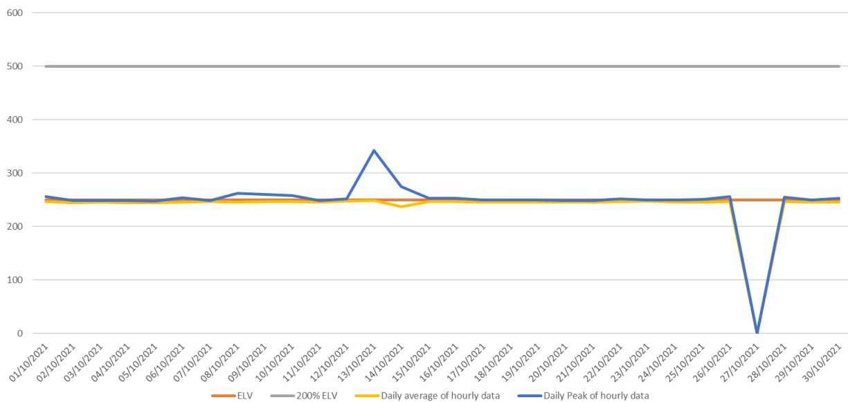
Summary of Nox emissions - Oct 2021
