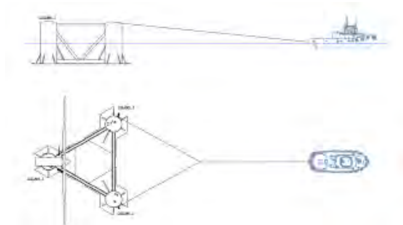
Figure 4.11: Towing out of WindFloat Unit to Offshore Array Site (source: PPI, 2019b)
