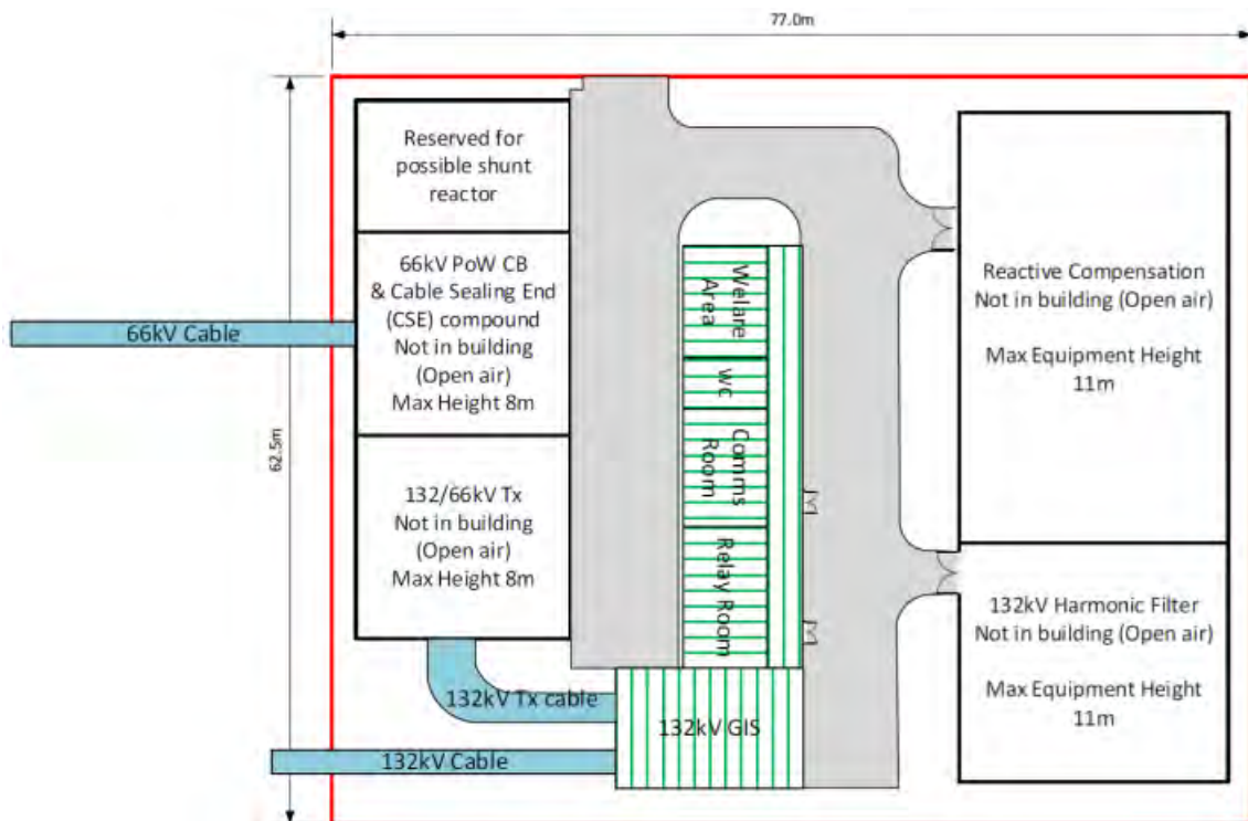
Figure 4.9: Indicative Substation Layout (source: JFMS, 2019)
