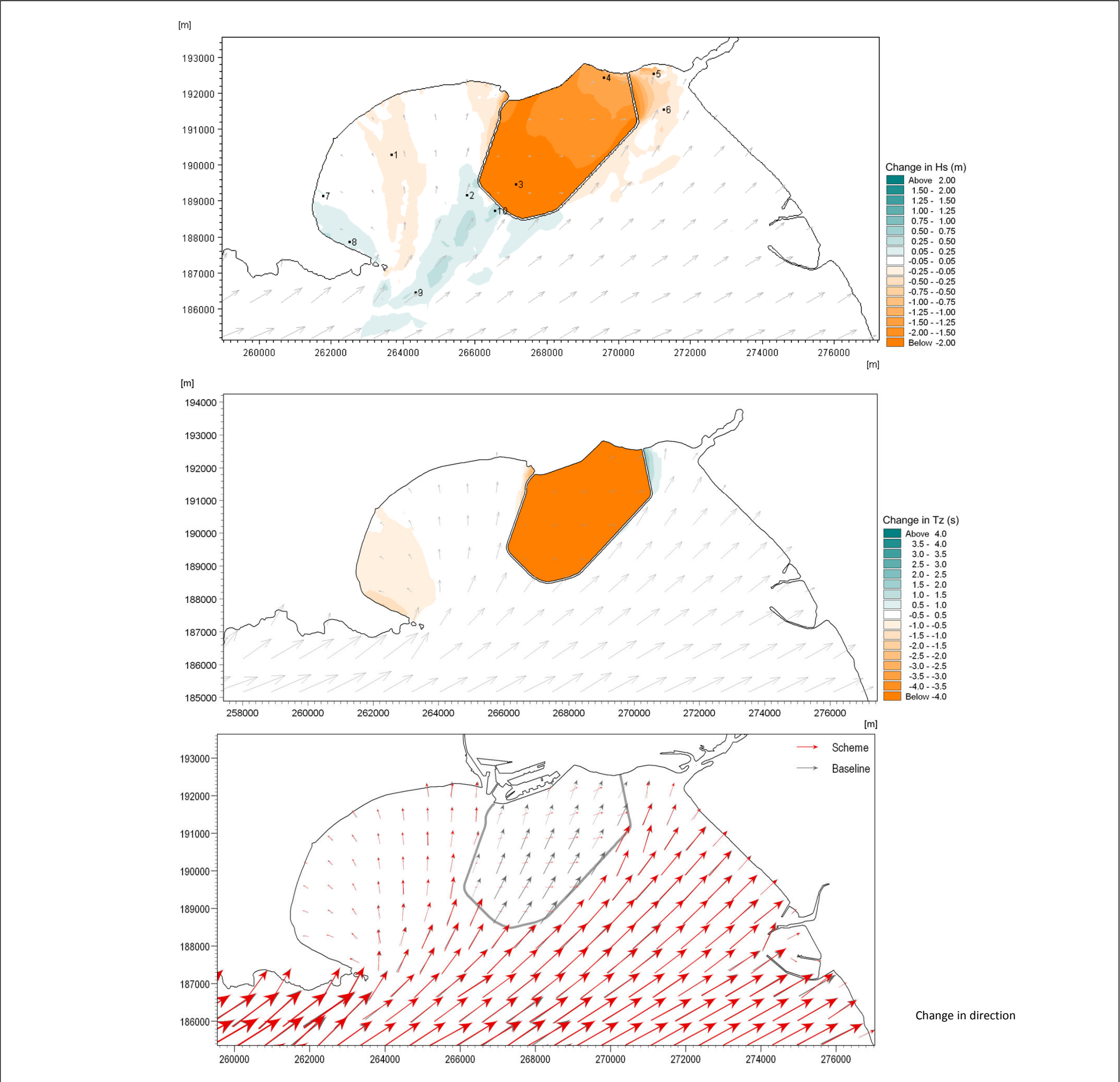
FIGURE 6.46 PREDICTED CHANGES TO WAVE PARAMETERS – 1 IN 10 YR SOUTH- WESTERLY WAVE
