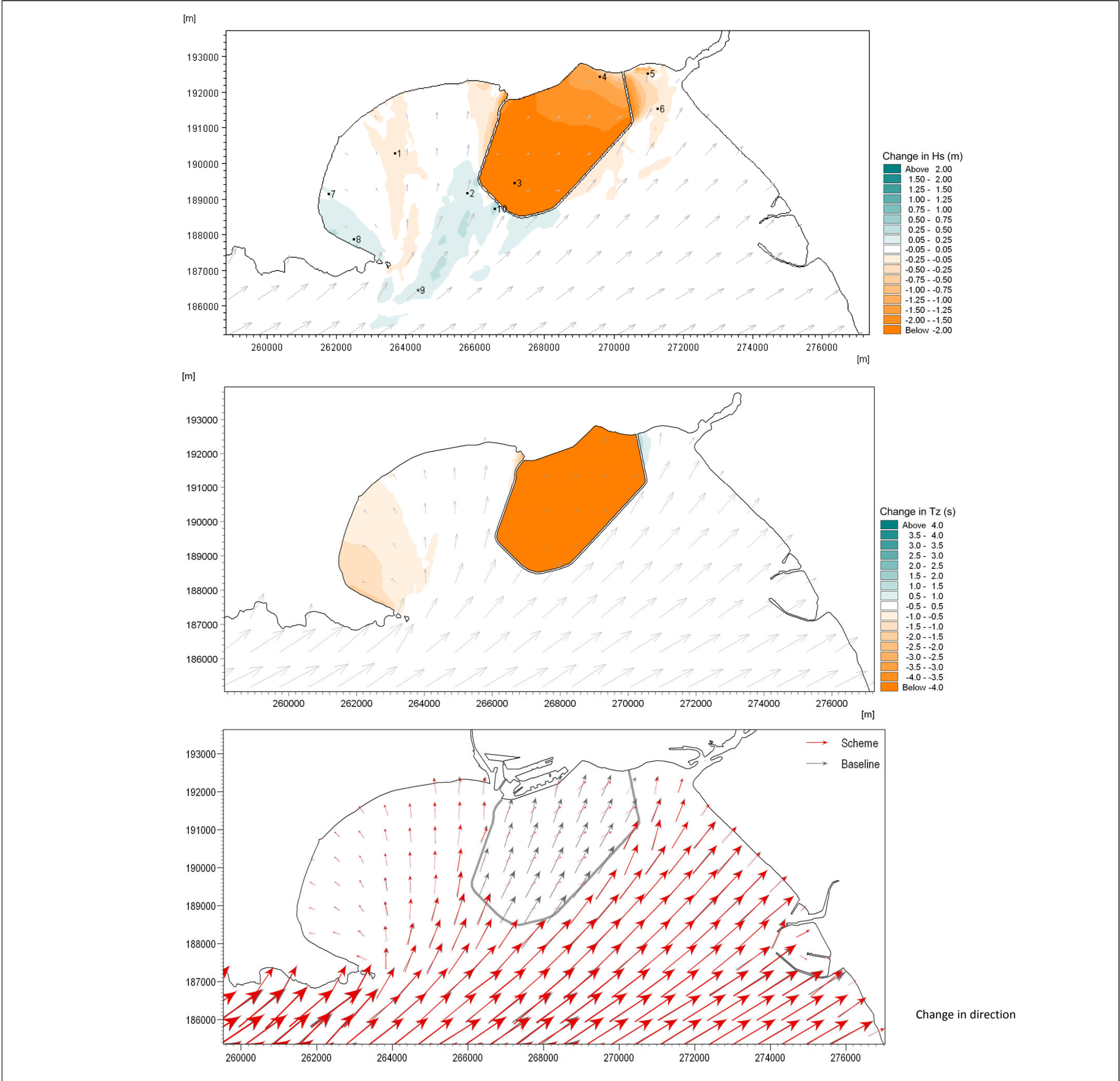
FIGURE 6.47 PREDICTED CHANGES TO WAVE PARAMETERS – 1 IN 20 YR SOUTH- WESTERLY WAVE
