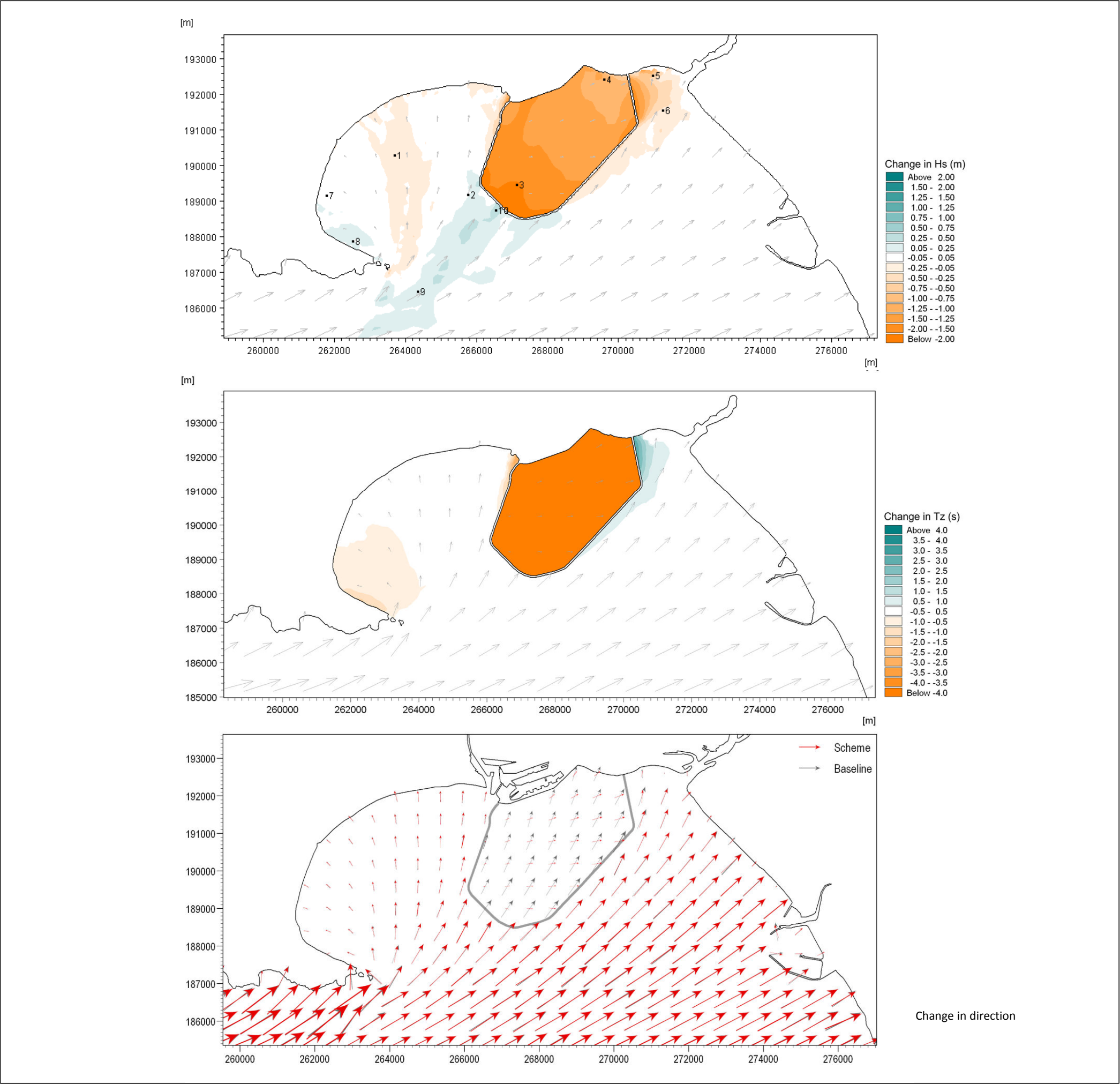
DRAWING TITLE FIGURE 6.45 PREDICTED CHANGES TO WAVE PARAMETERS – 1 IN 1 YR SOUTH- WESTERLY WAVE
