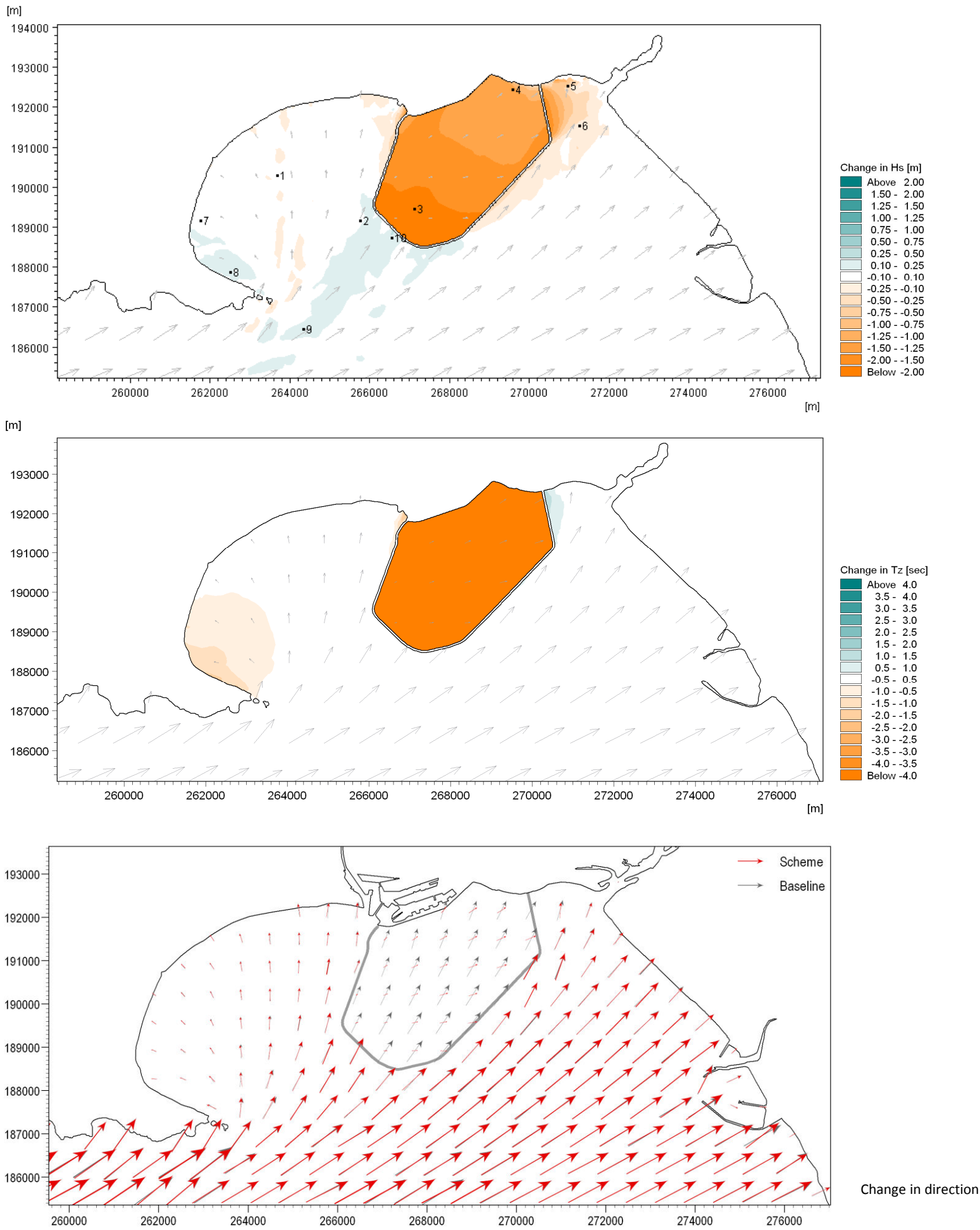
DRAWING TITLE FIGURE 6.44 PREDICTED CHANGES TO WAVE PARAMETERS – 10 IN 1 YR SOUTH- WESTERLY WAVE
