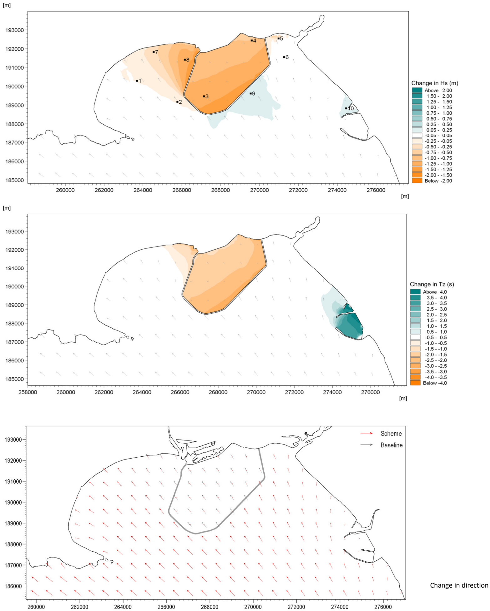
DRAWING TITLE FIGURE 6.49 PREDICTED CHANGES TO WAVE PARAMETERS – 1 IN 10 YR SOUTH- EASTERLY WAVE
