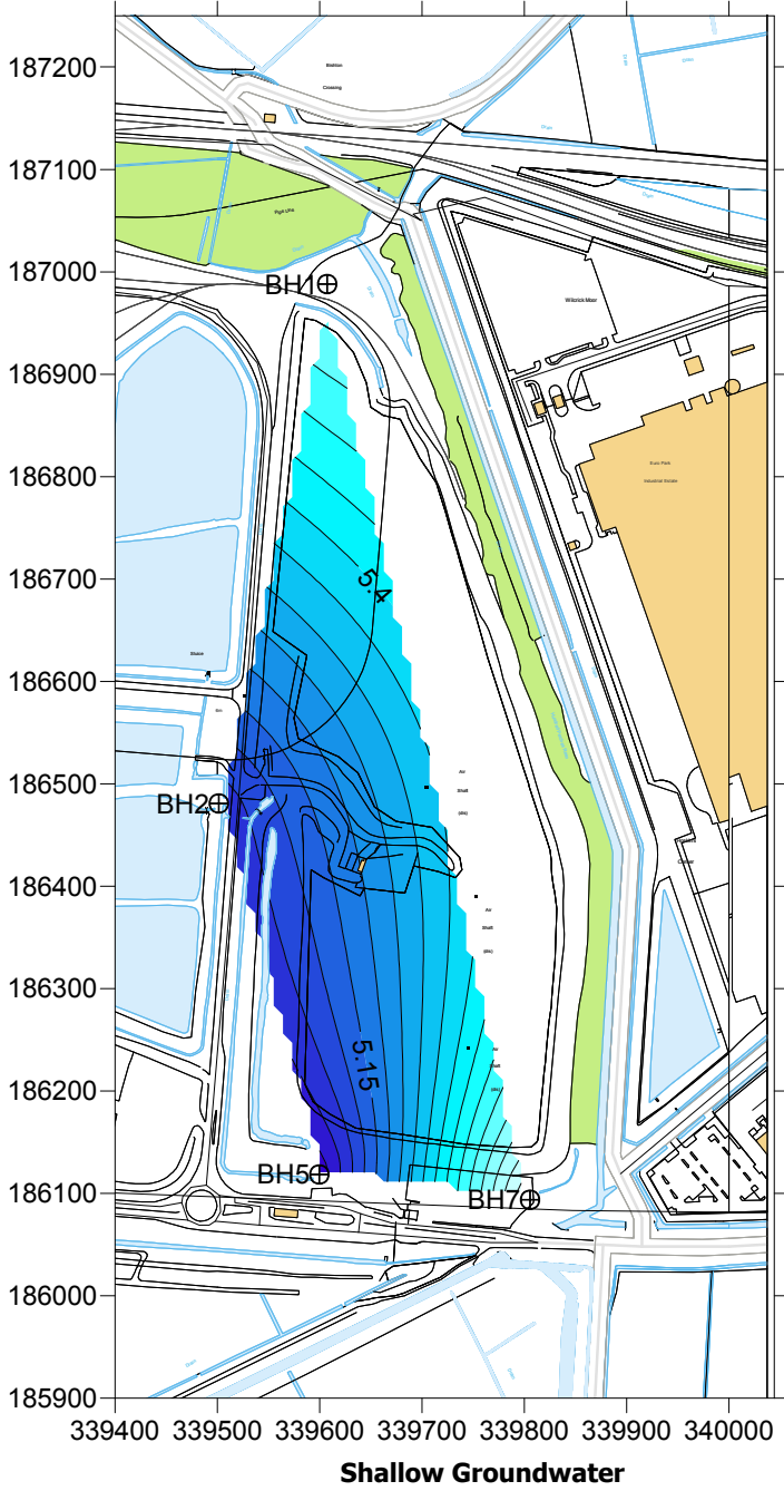
Figure 9 Recent Groundwater Elevations (mAOD)
