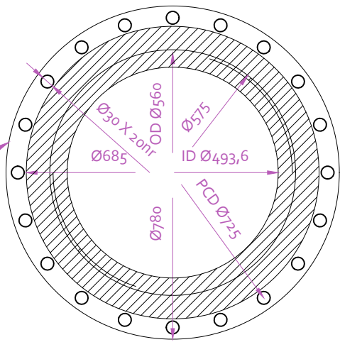
OUTFALL STUB END DETAIL-560mm OD HDPE
