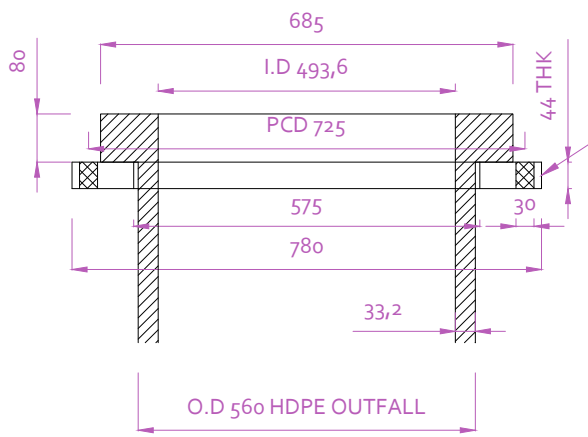
OUTFALL STUB END DETAIL- 560mm OD HDPE
