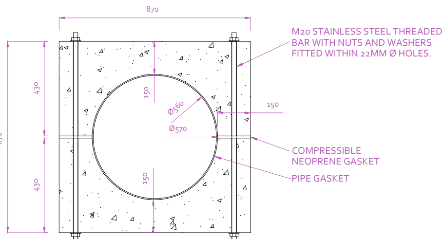
CONCRETE BALLAST COLLAR DETAILS
