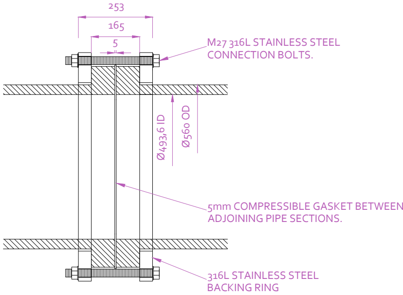
OUTFALL STUB ENDS CONNECTION DETAIL- 560mm OD HDPE
