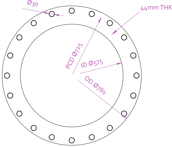
316L STAINLESS STEEL BACKING RING DETAIL- 560mm OD HDPE
