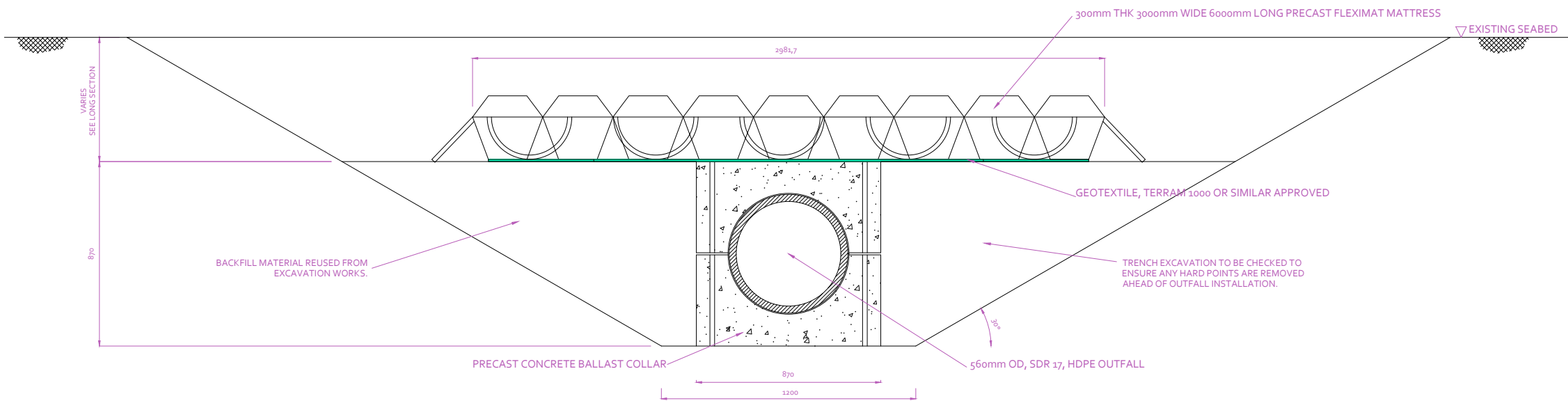
TYPICAL TRENCH PROFILE- SEABED
