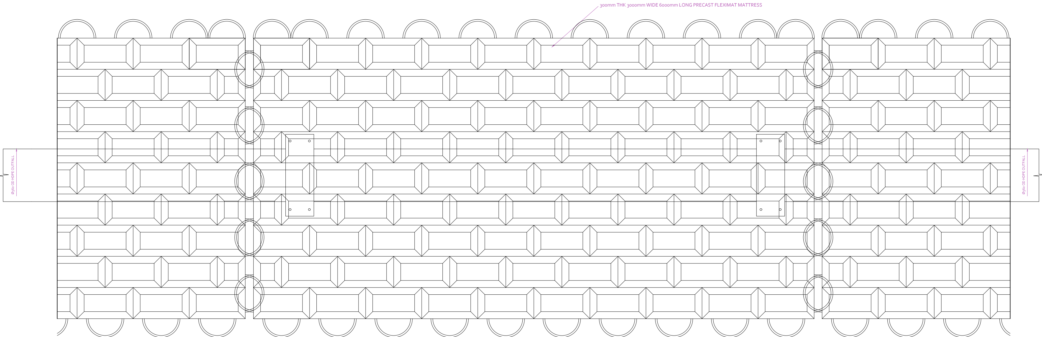
316L STAINLESS STEEL BACKING RING DETAIL- 560mm OD HDPE
