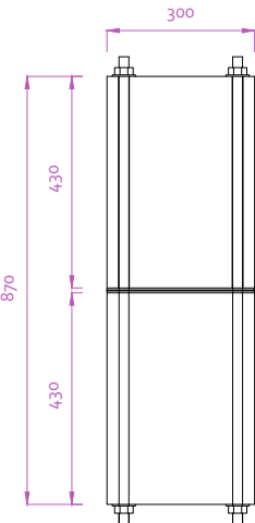
CONCRETE BALLAST COLLAR DETAILS
