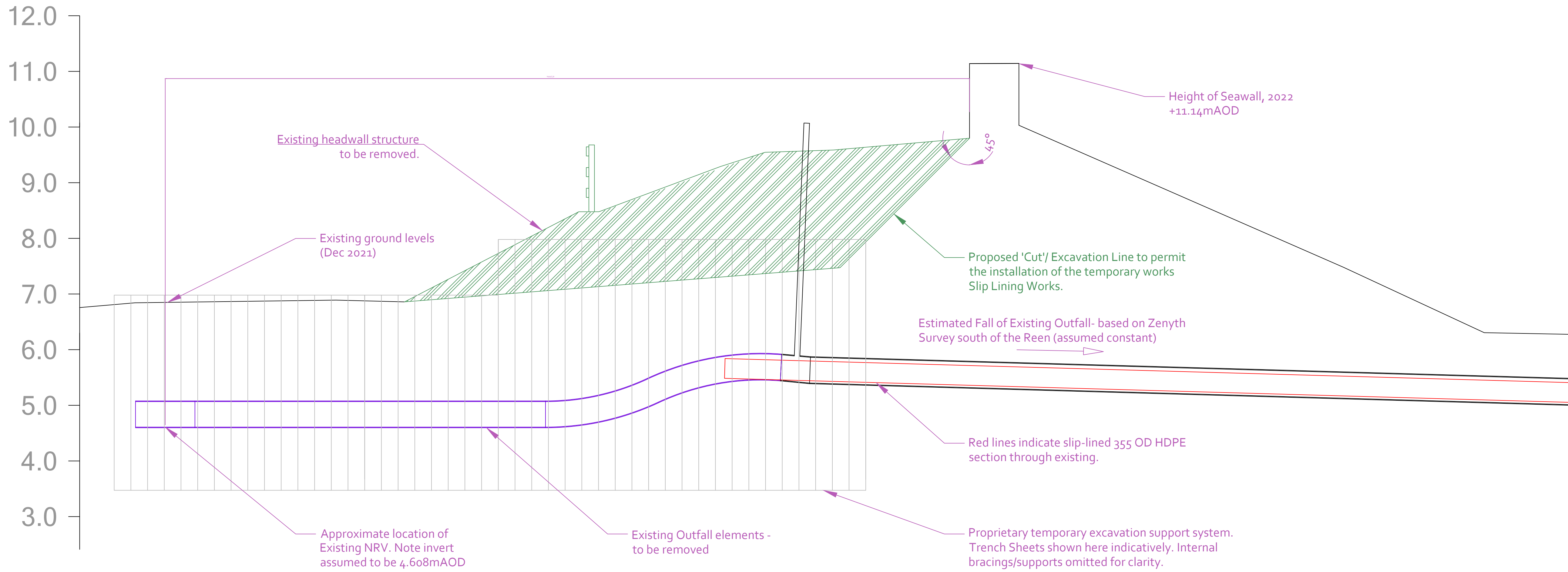
EXISTING CROSS SECTION DETAIL
