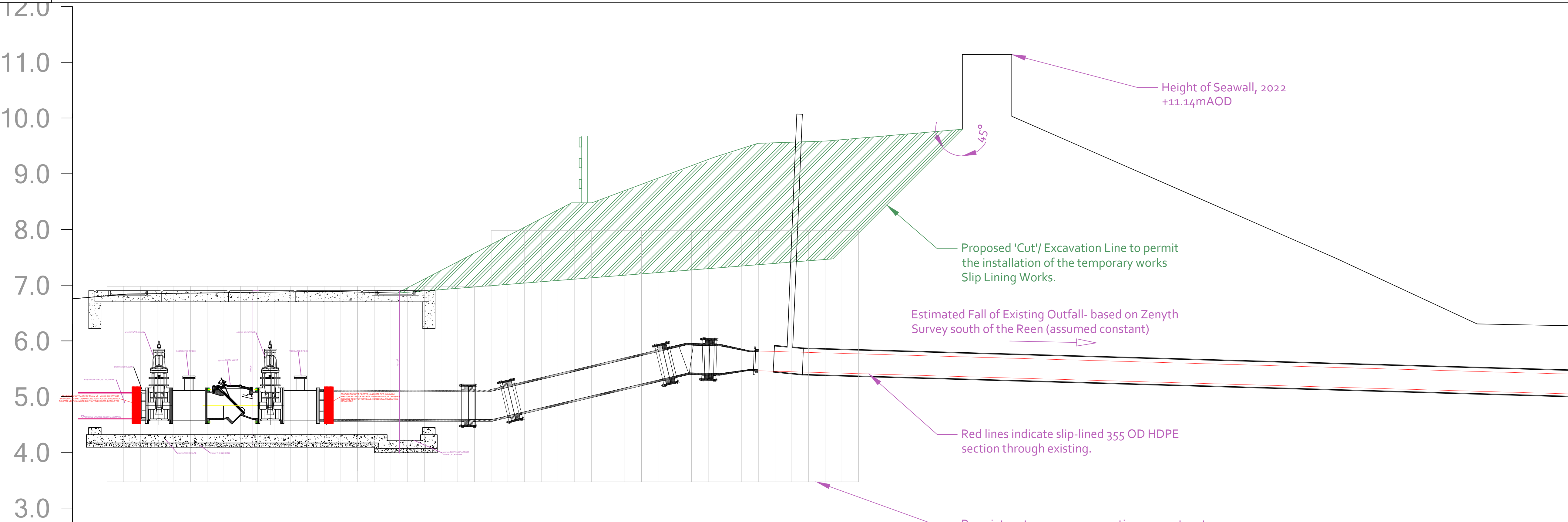
PROPOSED CROSS SECTION DETAIL See Drawing 1001 06 for further details
