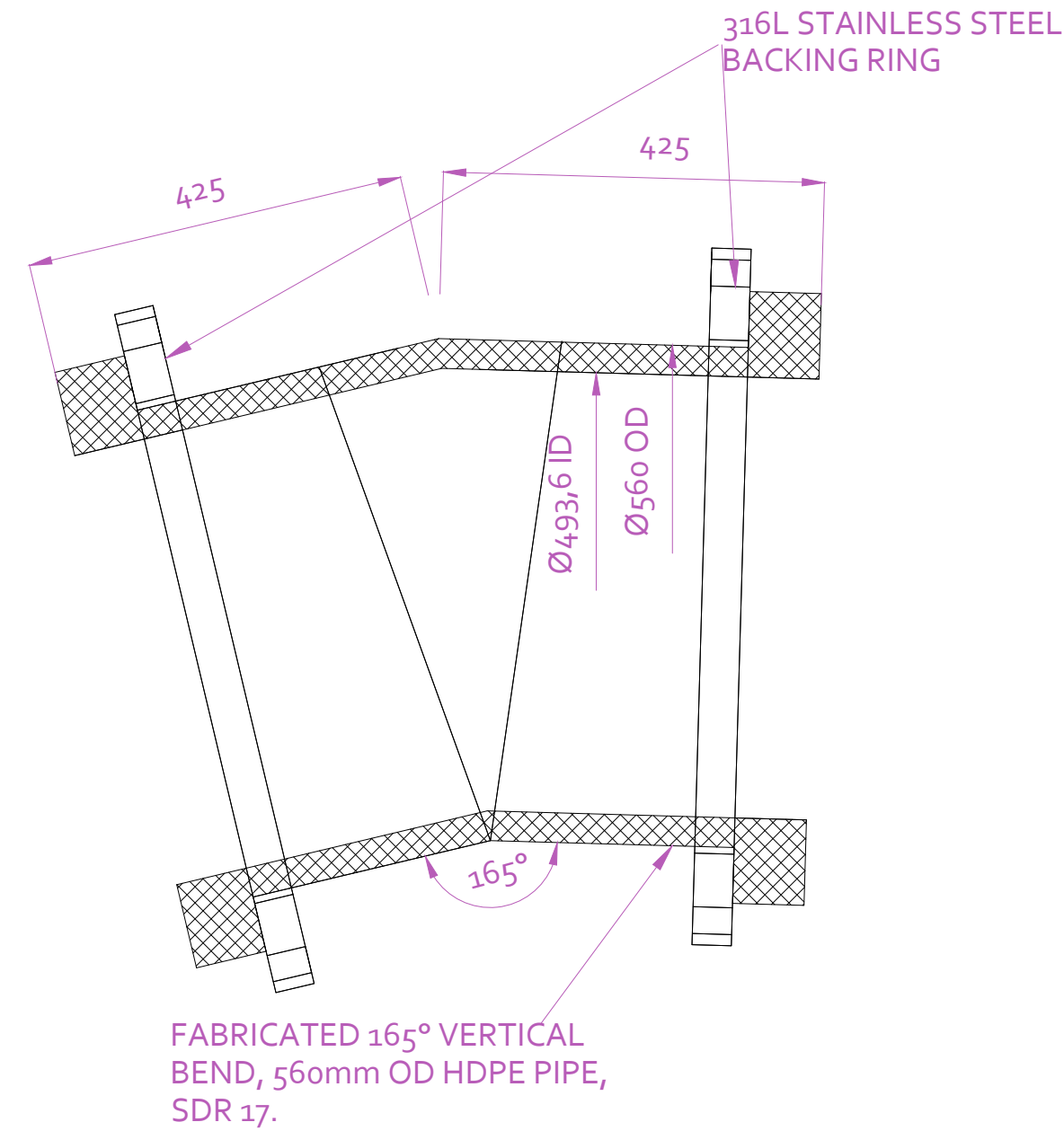
ITEM 3 - 1 NO. REQUIRED PROPOSED VERTICAL BEND DETAIL- 56mm OD HDPE SIDE ELEVATION
