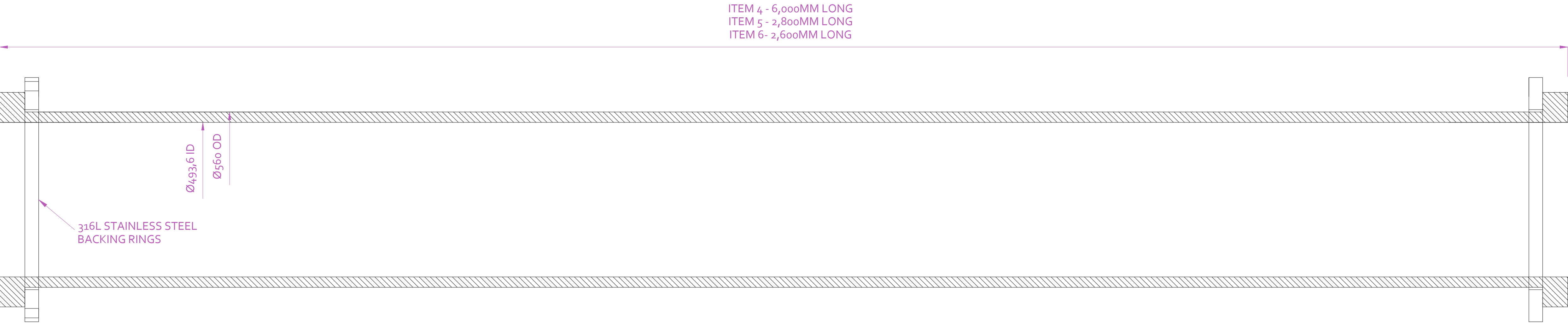
56mm OD HDPE STRAIGHT LENGTHS- 3 NR REQUIRED OF DIFFERENT LENGTHS (SEE ABOVE) CONNECTION DETAIL SIDE ELEVATION
