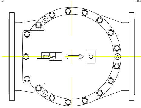
450mm Ø SWING FLEX CHECK VALVE PLAN VIEW
