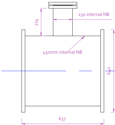
450mm Ø FABRICATED T PIECE SIDE ELEVATION
