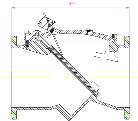
450mm Ø SWING FLEX CHECK VALVE SIDE ELEVATION
