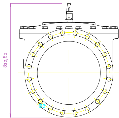
450mm Ø SWING FLEX CHECK VALVE FRONT ELEVATION
