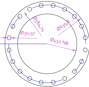
450mm Ø FABRICATED T PIECE FLANGE DETAIL
