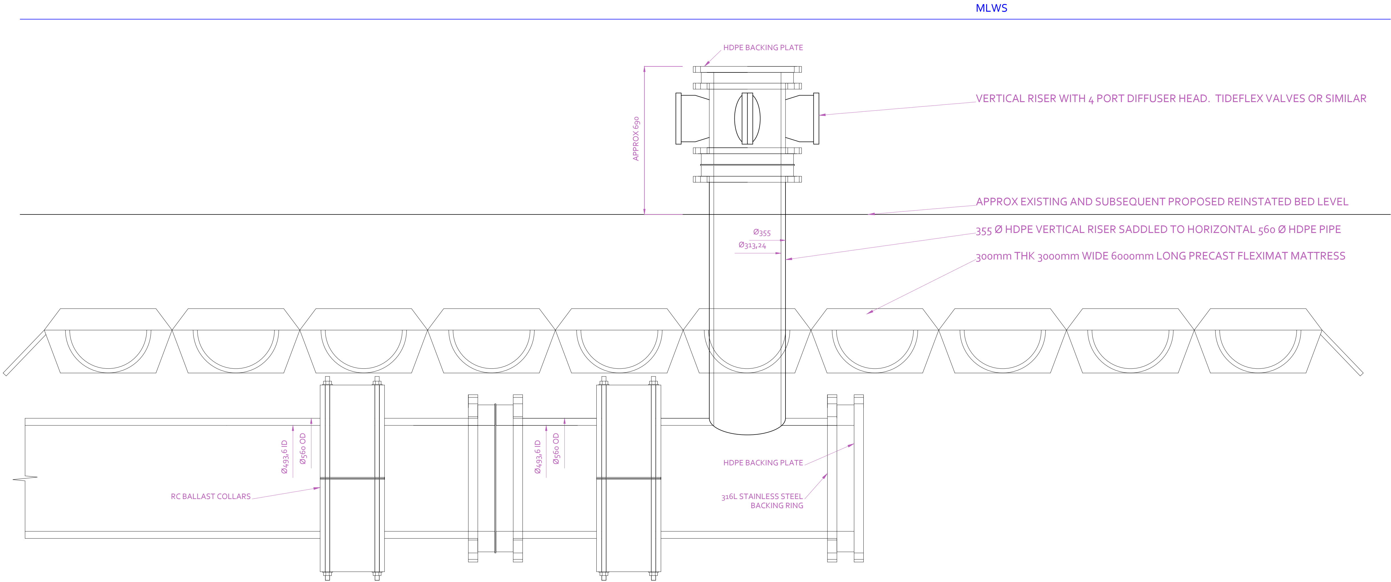
PROPOSED OUTLET DETAIL SIDE ELEVATION
