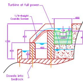
FRONT ELEVATION of FLOW-SPLIT NOTCH (A-A)
