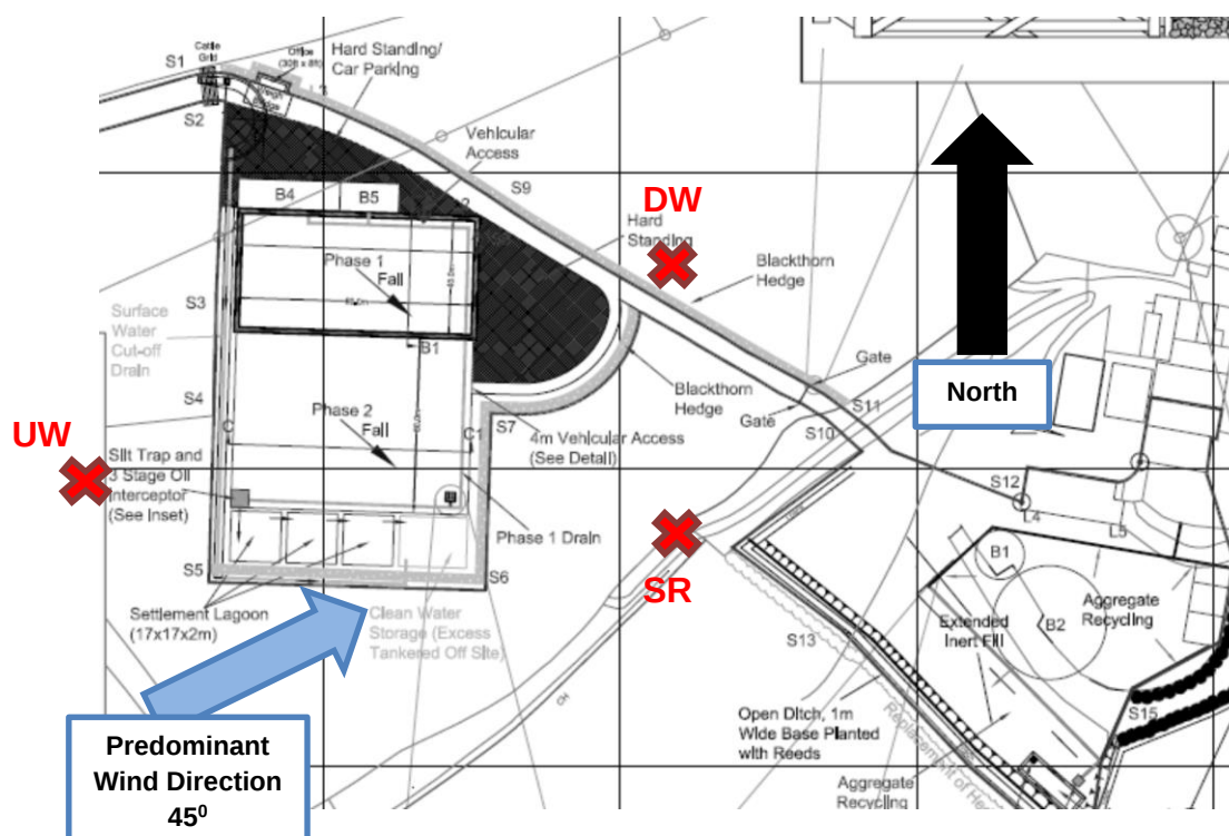
Figure 1 - Wind Direction and Sampling Points on 23/02/2017
