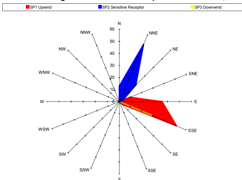
Figure 2: Wind Rose Illustrating Wind Patterns at Sample Locations SP1, SP2 and SP3.
