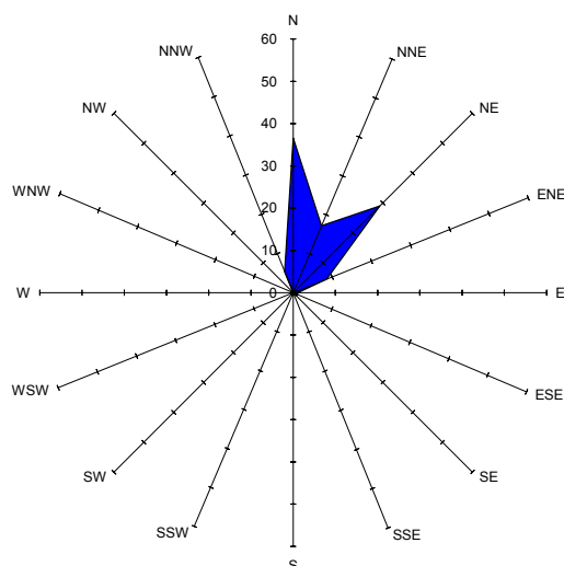
Figure 1: Wind Rose Illustrating Mean Wind Direction from the Northeast.
